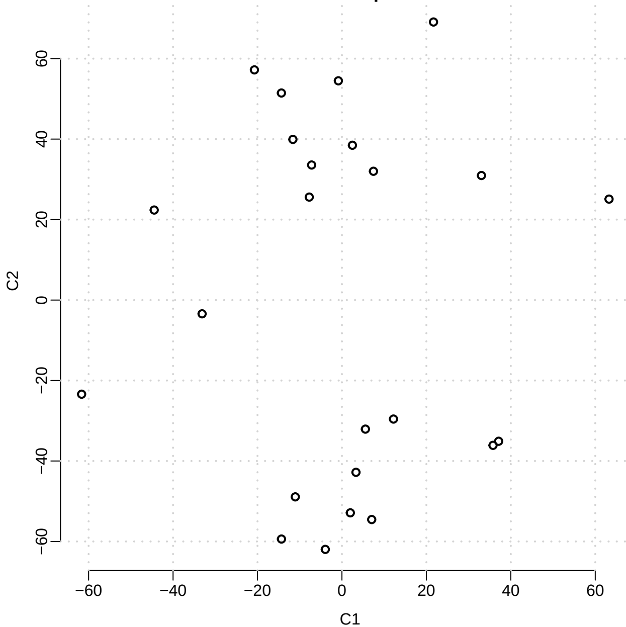
OPLS scores per m/z
