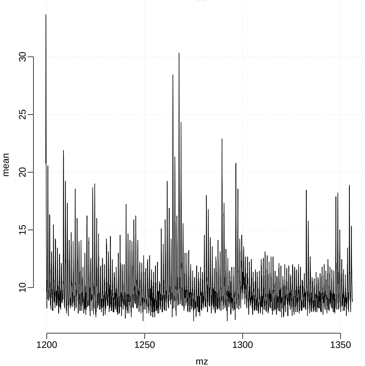
Average spectrum mean
