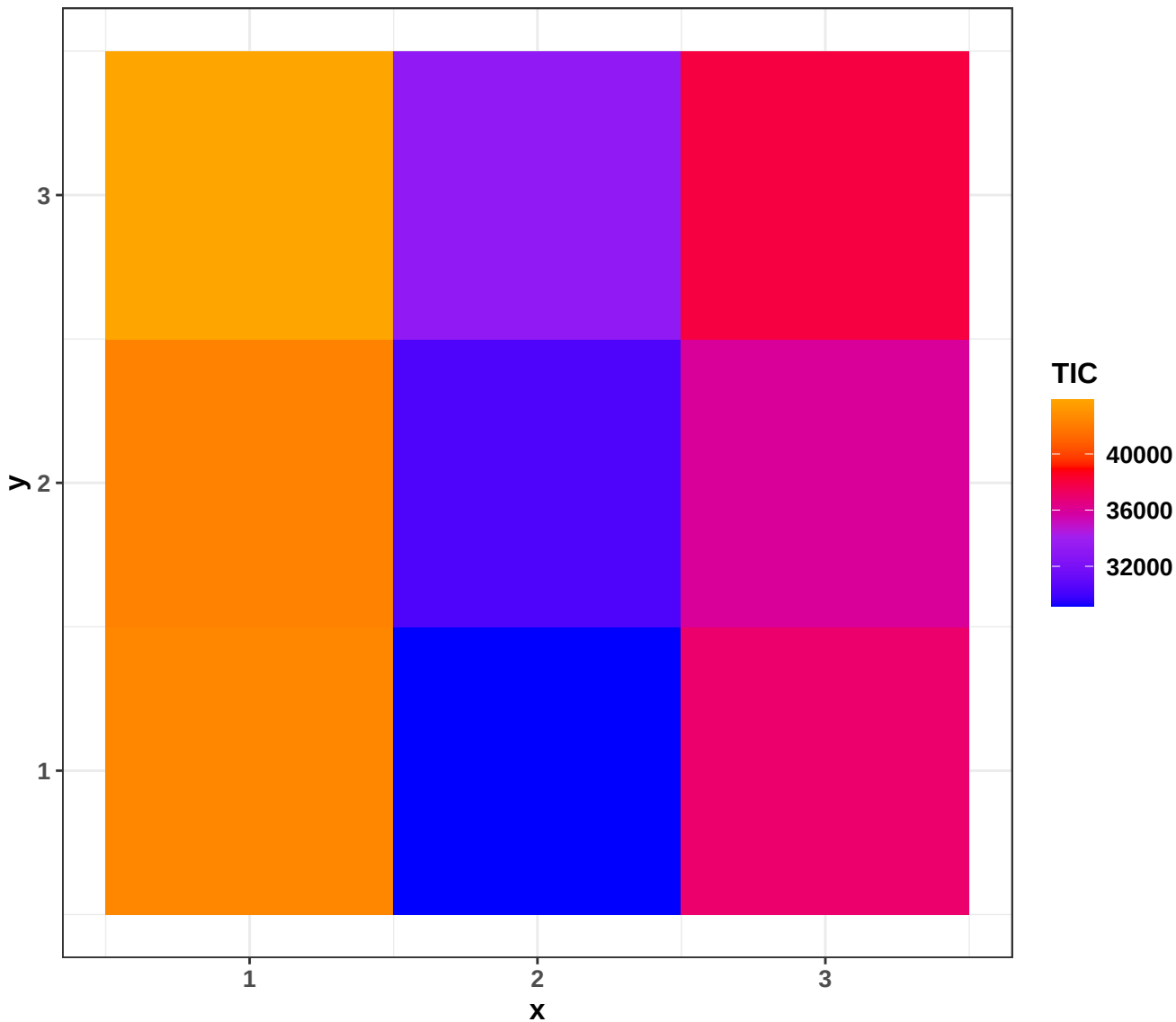
Total Ion Current
