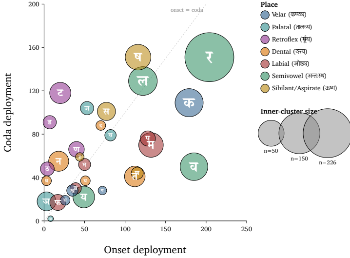
Figure 6: Valency map: onset \times coda scatter of Dhātupāṭha deployment, with bubble size encoding inner-cluster activity and color encoding place of articulation. Onset specialists ( ka , va , pa , ta ) sit far right; coda specialists ( ja , sa , ḍa , ṭa ) sit high up; balanced consonants ( la , bha , cha ) sit near the dashed onset = coda diagonal. Ra (र) appears as the largest bubble — its inner-cluster activity makes it the universal bonder, visible at a glance. The retroflex closure pattern is also visible: ṭa (ट), ḍa (ड), ṇa (ण), ṣa (ष) cluster in the high-y / low-x quadrant.
