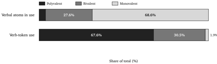
Figure 37: Reactivity tiers by atom share and actual Sanskrit use.
