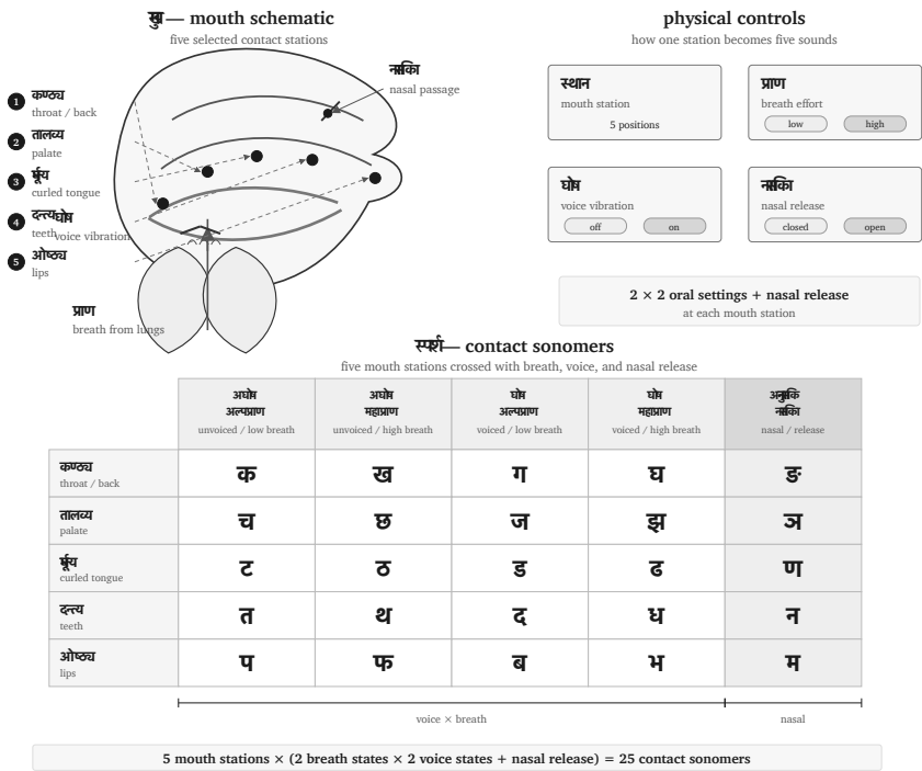
Figure 5: Figure 8.3 — Control-panel view of the sparśa matrix: five mouth-stations crossed with breath, vocal-cord vibration, and nasal release.
