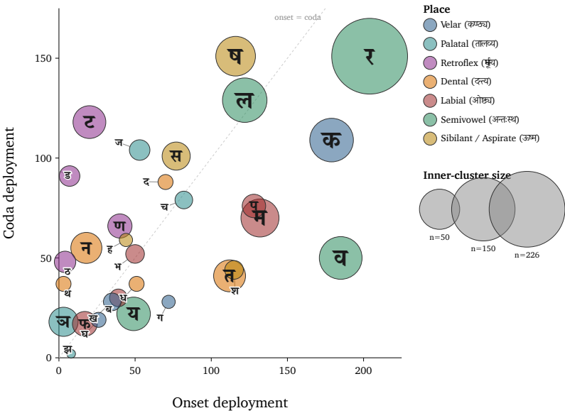
Figure 12: Position-role map of consonants across single- akṣara atoms.
