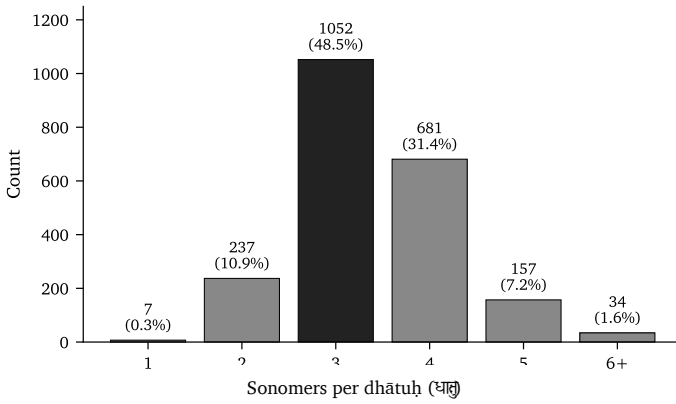
Figure 9: Sonomer-count distribution across the 2,168 dhātavaḥ .
