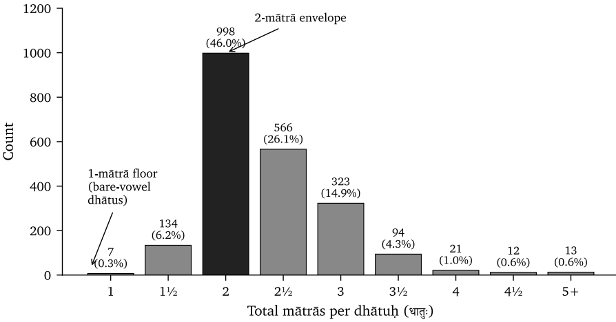
Figure 35: Distribution of the 2,168 dhātavaḥ across mātṛā values.
