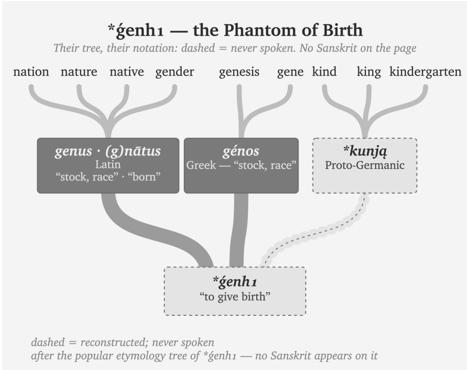
Figure 19.4 — *ǵenĥ₁ — the Phantom of Birth. Another popular tree, trimmed the same way — their branches, their notation, nothing added: dashed = never spoken. No Sanskrit in the tree.
