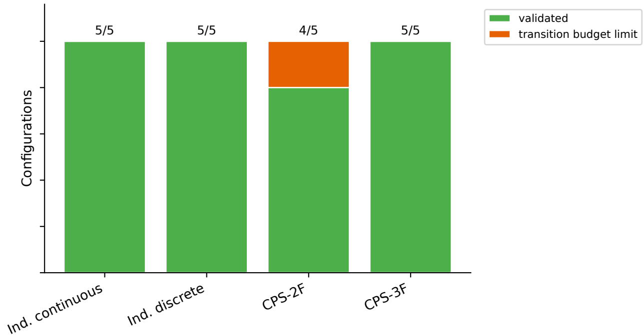
Hurricane (5 configurations/method)
