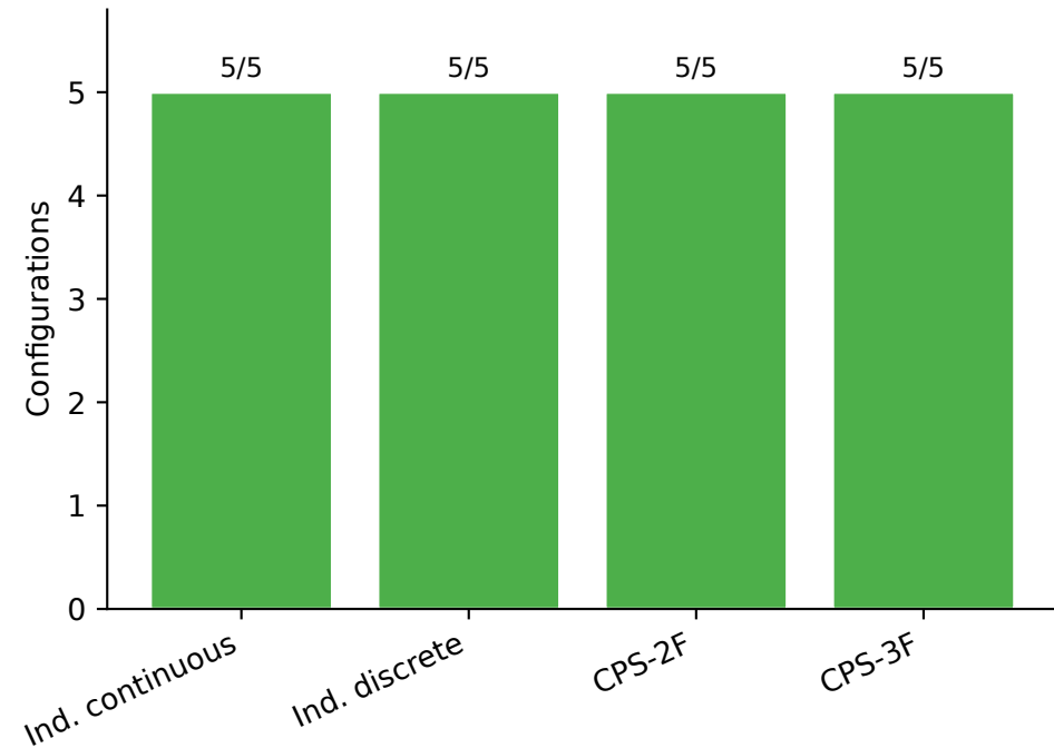
Protein (5 configurations/method)
