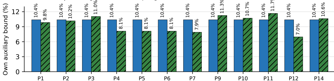
(a) Proteins | existing w=16 subsampling
