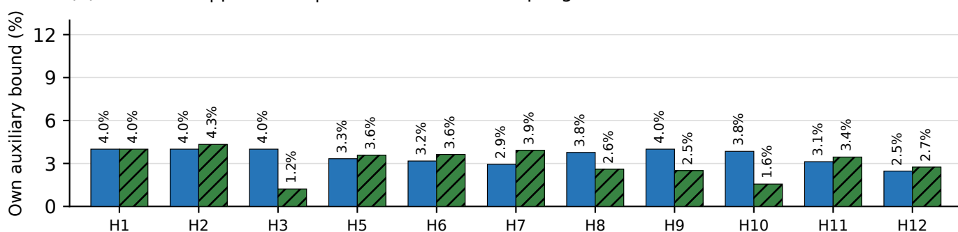
(b) Hurricanes | panel 1/3 | no additional subsampling
