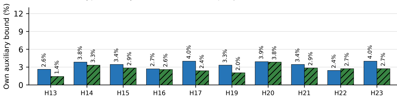
(c) Hurricanes | panel 2/3 | no additional subsampling
