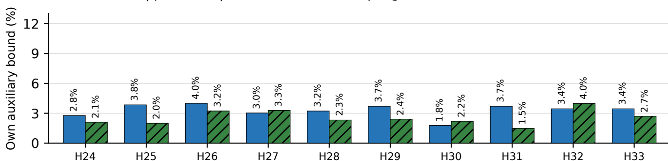
(d) Hurricanes | panel 3/3 | no additional subsampling
