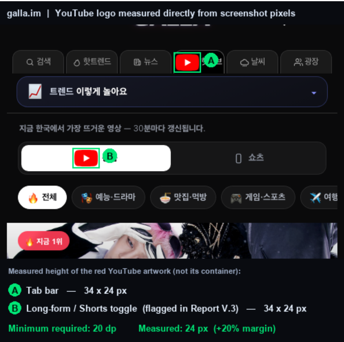
Figure 1 — galla.im/search?tab=hot, captured after deployment 0820102.
