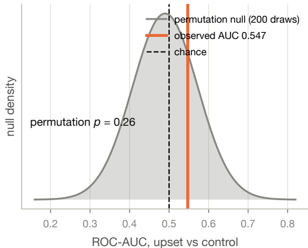
(a) classification is at chance
