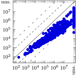
Sat clauses
