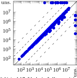
Sat clauses
