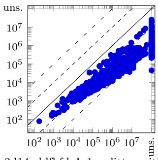
Sat clauses
