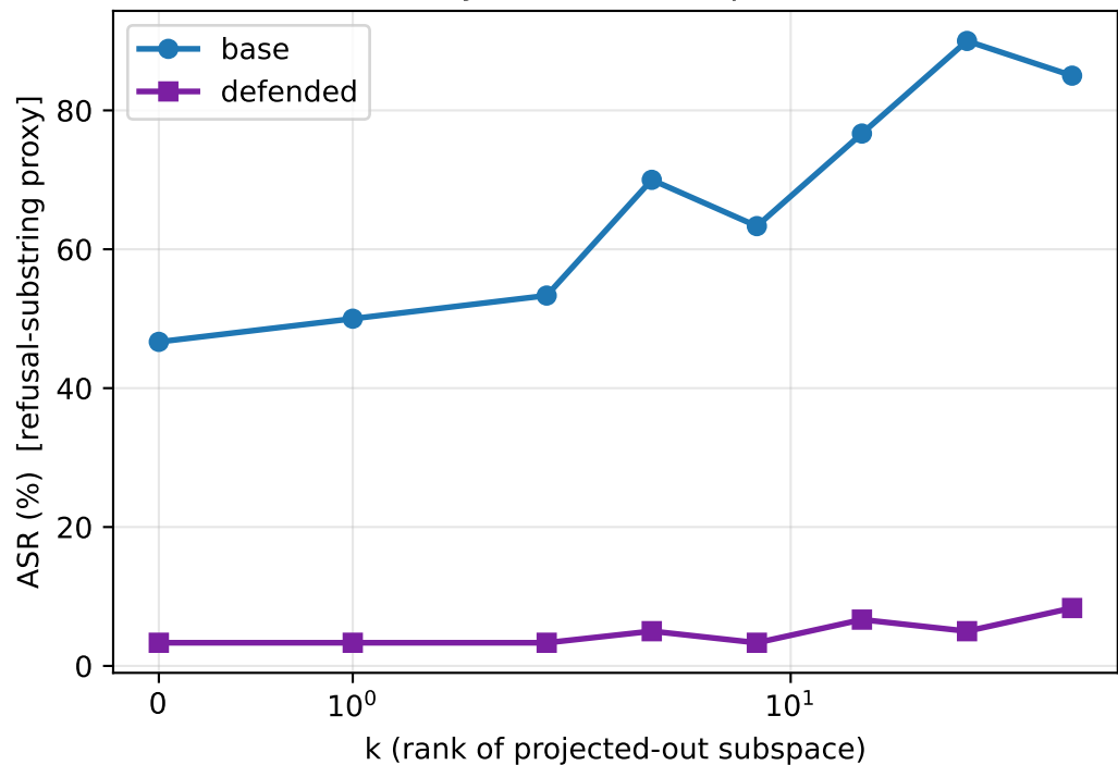
layer 16 (50% depth)
