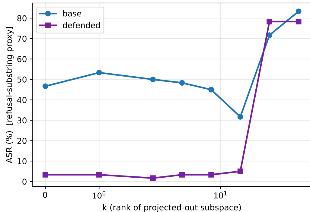
layer 10 (31% depth)
