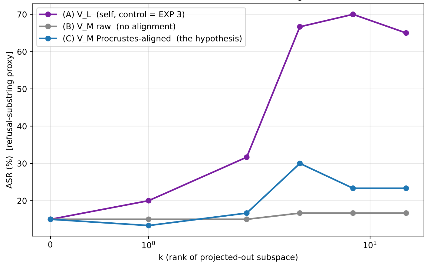
Remote un-defense on defended Llama-3 @ L16 (n=60)
