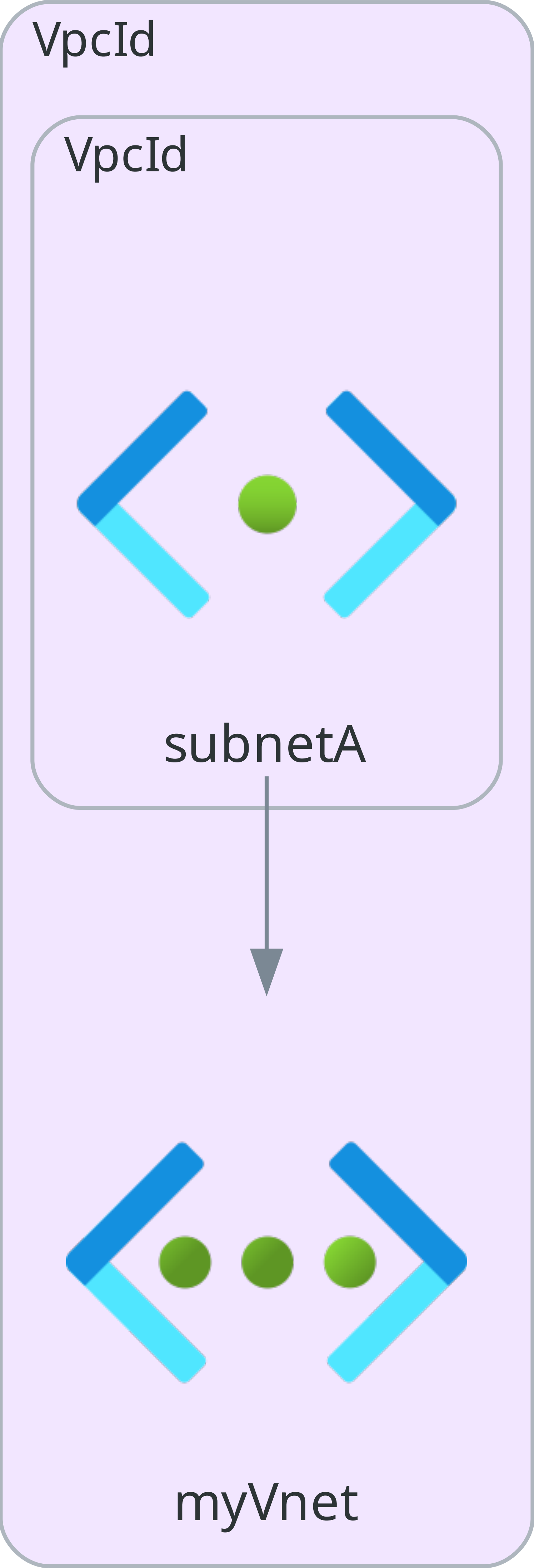
Azure Infrastructure: simple_vnet.bicep
