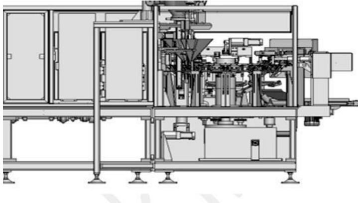
Pick fill seal for standee spout & non spout
