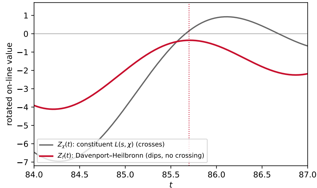
D2b: the phantom on the line — dip 0.357 at t = 85.70
