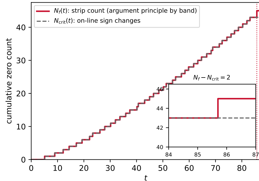
deficit on [0, 87] : N_f = 45 , C = 43 ; control L(s, \chi) : 45 = 45
