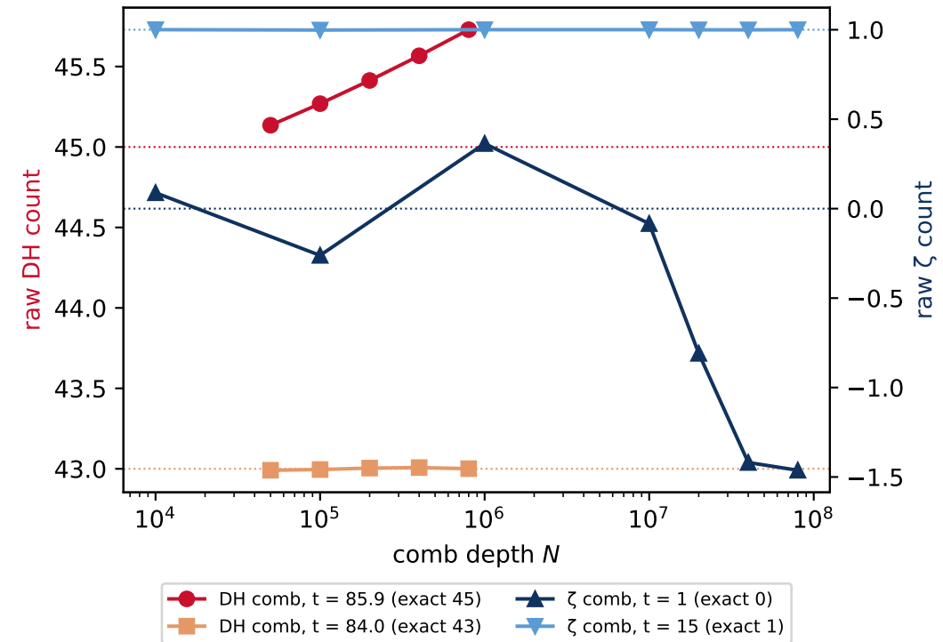
D2d/D2e: the raw count does not settle near a singularity
