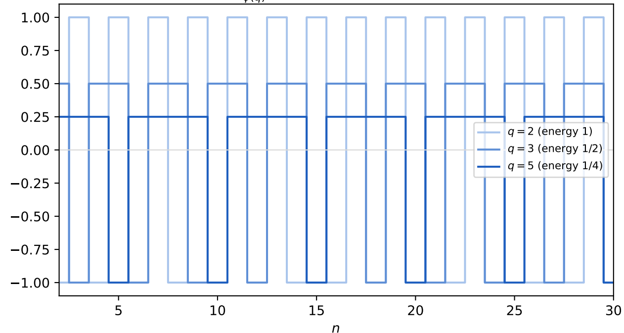
units-chart modes \frac{\mu(q)}{\varphi(q)} c_q in energy order (antipode q = 2 first)
