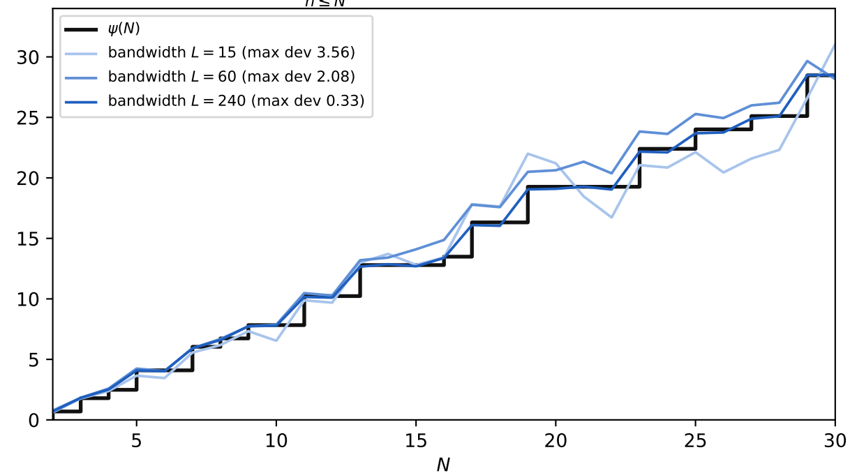
E1c: \Psi_L(N) = \sum_{n \leq N} \frac{n}{\varphi(n)} R_L(n) from L units-chart modes
