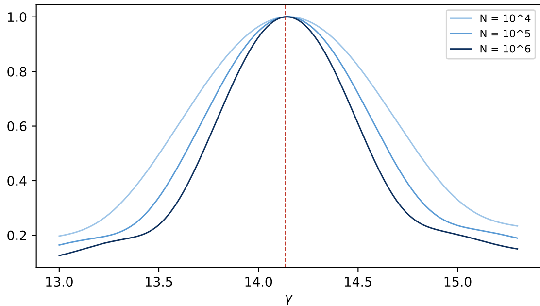
peak at \gamma_1 sharpens with depth, width \sim 2\pi/\log N
