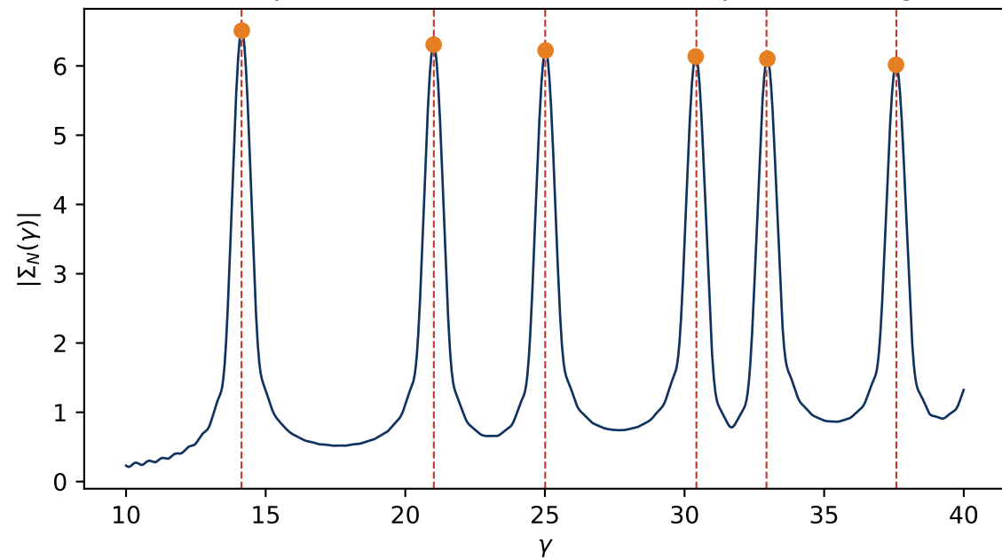
C1: scale-spectrum of the comb, N = 10^6 (peaks vs heights)
