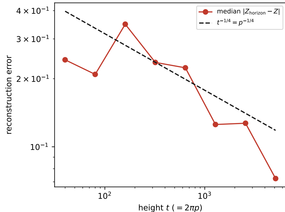
B2: residue \propto p^{-1/4} (slope -0.24)
