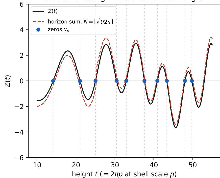
B4: de-framing = finite Riemann-Siegel
