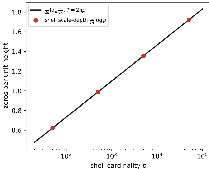
B1: zero density = shell scale-depth [chart]
