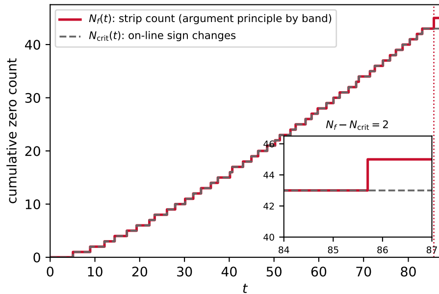
deficit on [0, 87] : N_f = 45 , C = 43 ; control L(s, \chi) : 45 = 45
