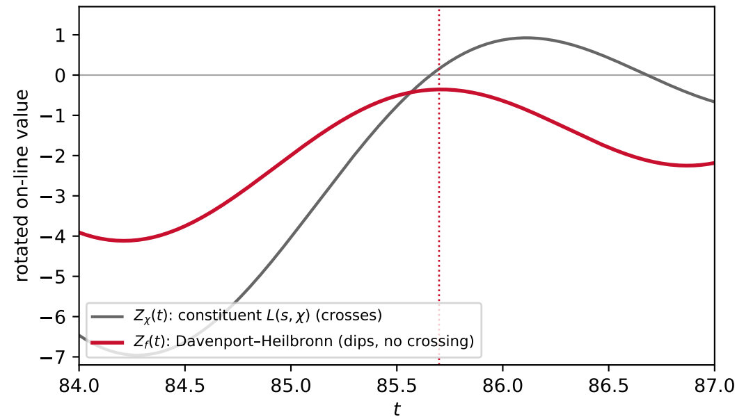
D2b: the phantom on the line — dip 0.357 at t = 85.70
