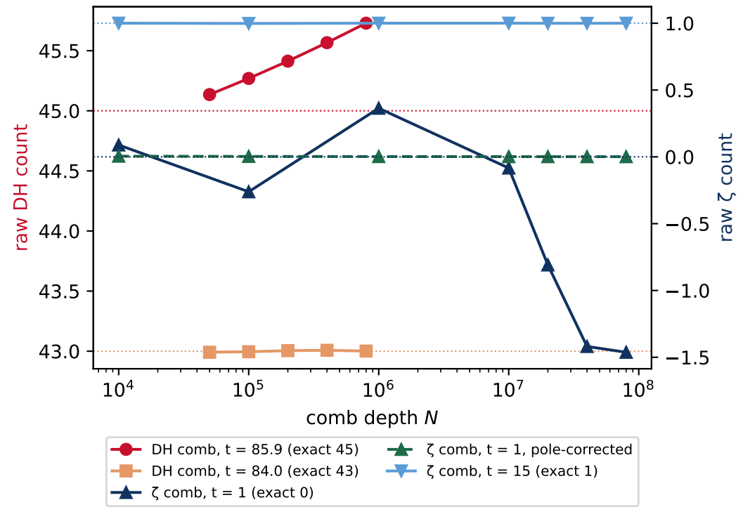
D2d-D2f: the raw count near a singularity, and the pole-corrected count
