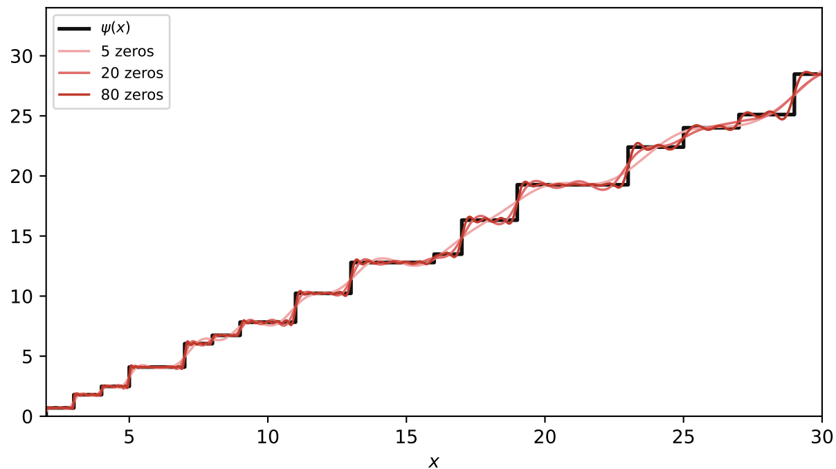
classical: \psi(x) from M zeros
