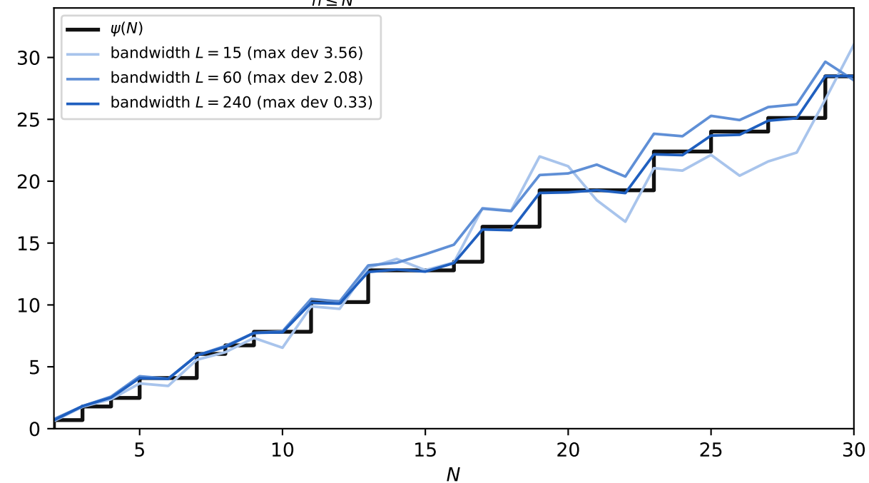
E1c: \Psi_L(N) = \sum_{n \leq N} \frac{n}{\phi(n)} R_L(n) from L units-chart modes
