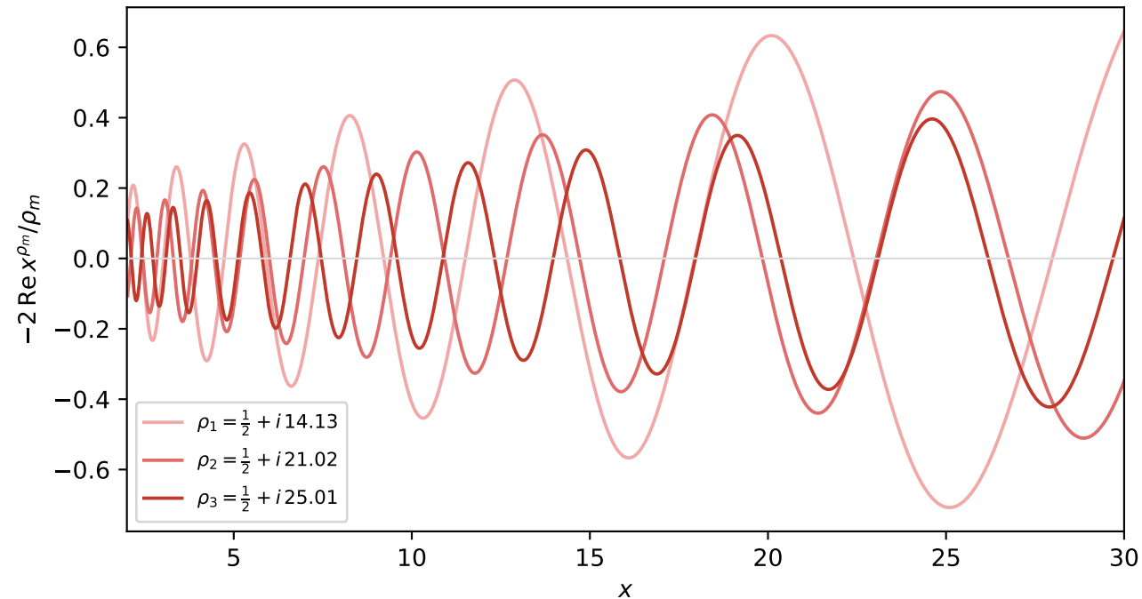
classical spectral modes: the zeros
