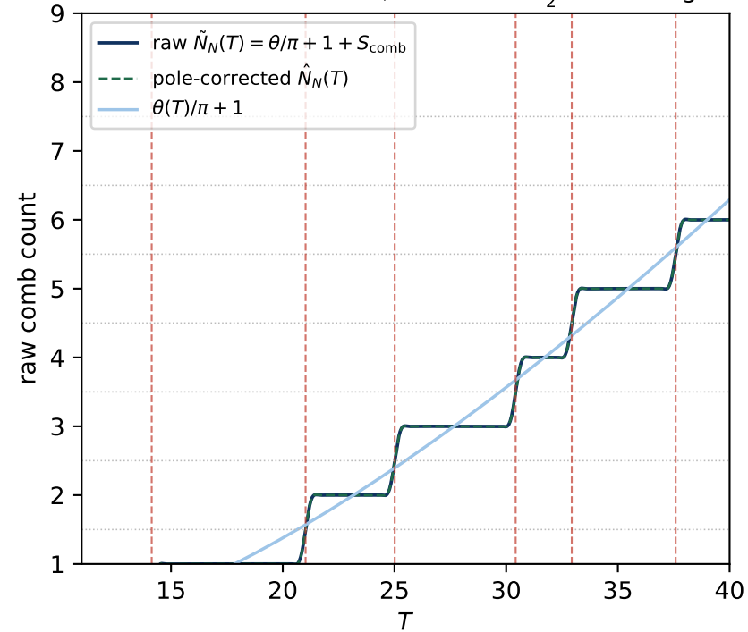
C2/C2b: secular condition, count = n - \frac{1}{2} at the heights
