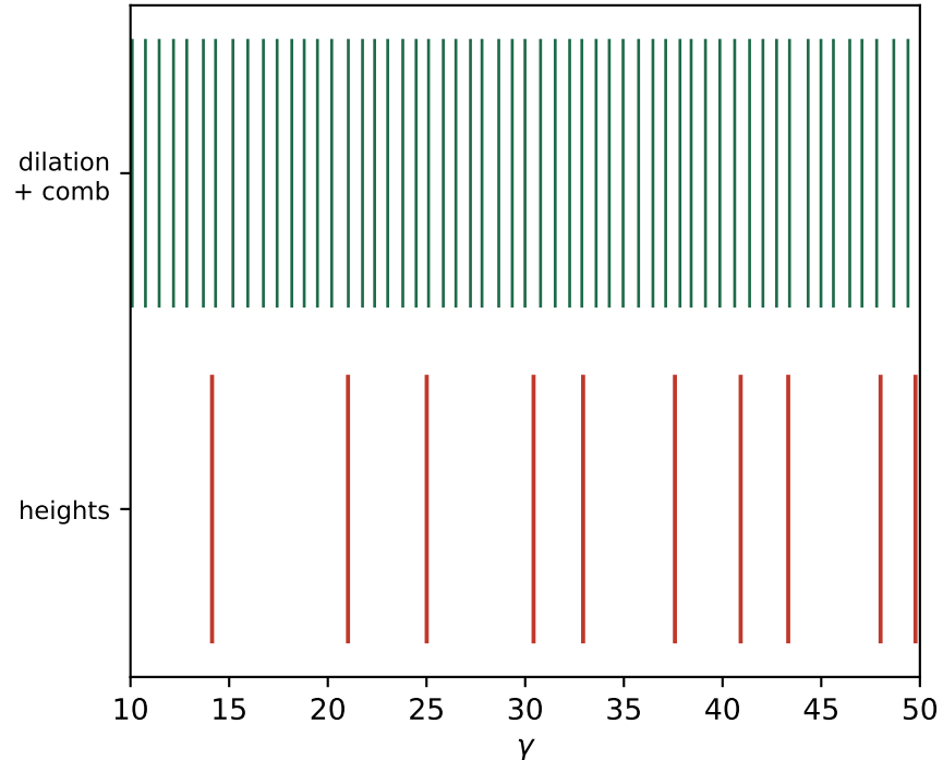
C5: additive injection is gauge-trivial
