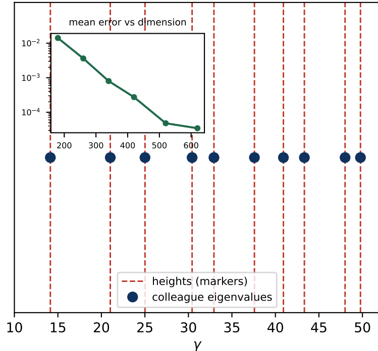
C3: colleague matrix (corrected), dim 520, mean err 4.8e-05
