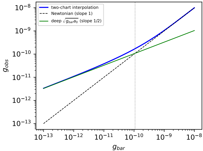
Radial acceleration relation
