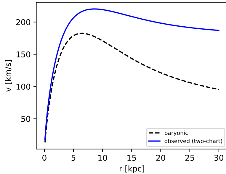
Rotation curve (exp. disk)
