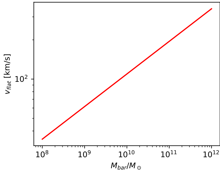
Baryonic Tully-Fisher (slope 0.25)
