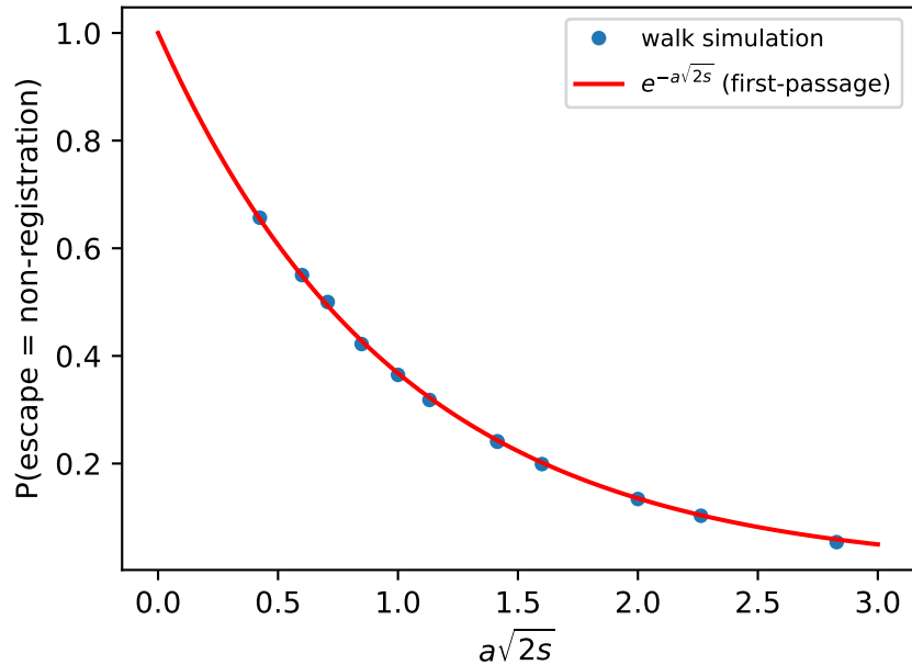
Meridian first-passage law
