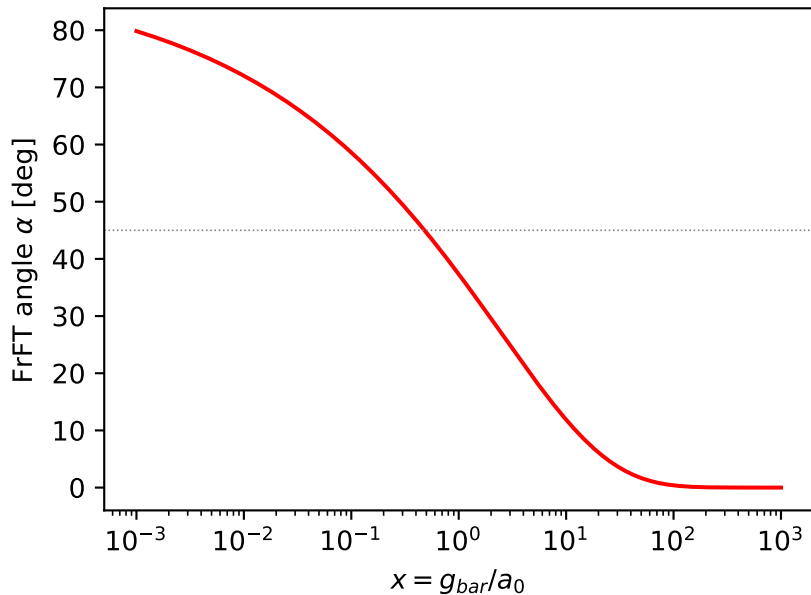
Chart angle: \sin^2 \alpha = e^{-\sqrt{x}} (0=space, 90=spectrum)
