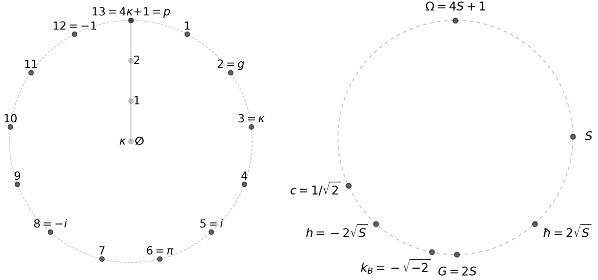
Figure 4: The two registers at the smallest admissible scale, (p, \Omega) = (13, 233) [33]. Subject (left): the shell \mathbb{F}_{13} a frame derives internally (generator g = 2 , capacity \kappa = 3 , quarter-turn i = 5 , half-period \pi = 6 , with -i = 8 , -1 = 12 , and the wrap point p \equiv 0 carrying its framed label); the radial axis holds the shell's information capacity. Carrier (right): \Omega = 233 , capacity S = 58 , displaying the residue pairs whose unit-face magnitudes the observer registers as the physical constants: G = 2S = 116 exact at the half-cycle; the root pair of -1 is \{89, 144\} , the \{h, h\} pair, both members marked; c and k_B shown by the representatives 159 ( c^2 \equiv 2^{-1} ) and 124 ( k_B^2 \equiv -2 ), pair partners 74 and 109. Marks are representative-convention data; the pairs are the Carrier facts: the flags are the content, the magnitudes their representative face, the physical-magnitude reading living in [33].
