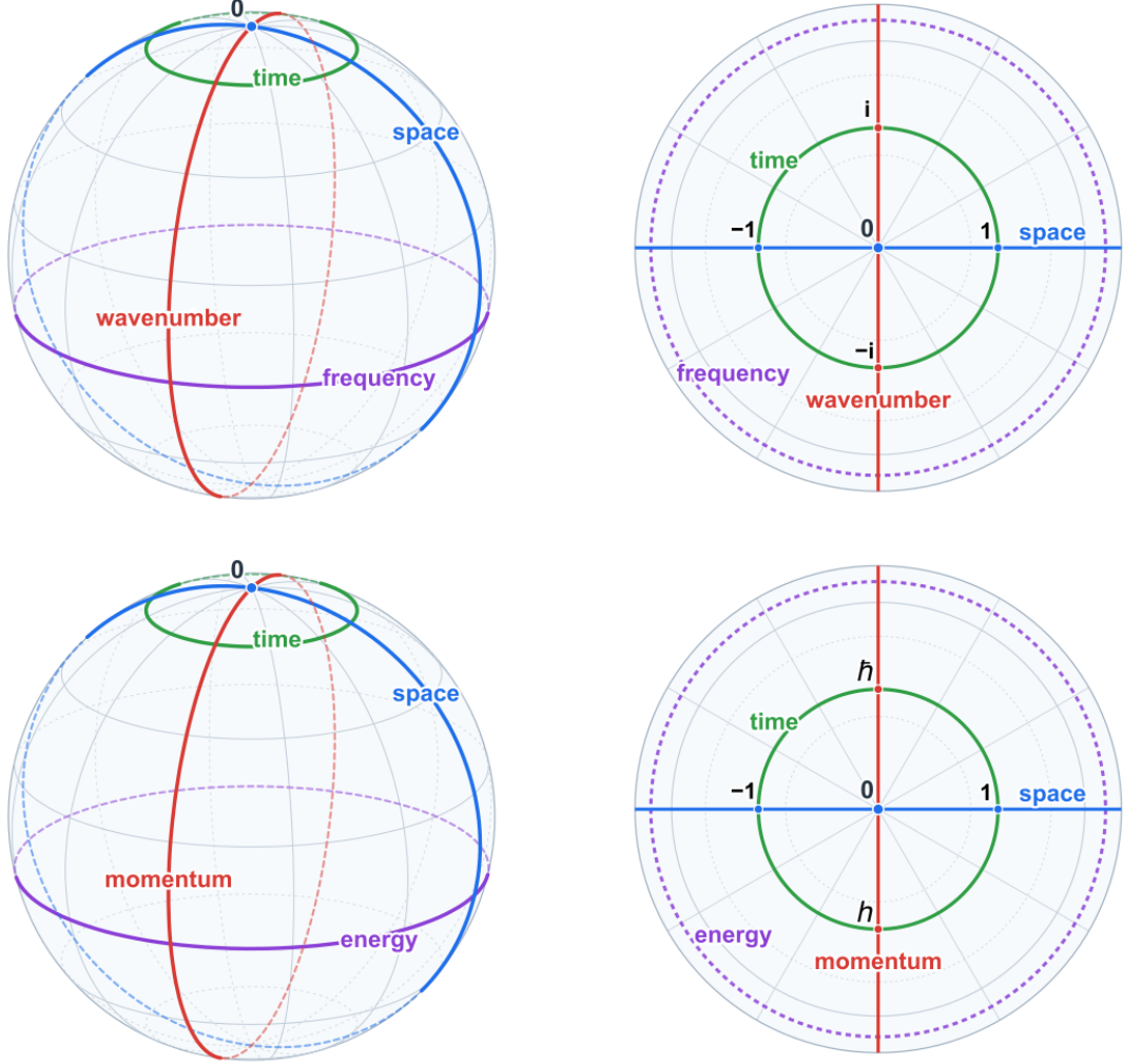
Figure 3: The four representation domains of a framed shell, in both registers [33]. Subject register (top): space (the prime meridian, blue) and wavenumber (red), the transverse additive-Fourier pair; time (green) and frequency (purple), the longitudinal multiplicative-Fourier pair, the drive running along time; left the orbital sphere with the origin at the pole, right the observer's chart with the cardinal residues 0, \pm 1, \pm i , the four counts flag-free and unitless relative to the frame's own anchors. Carrier register (bottom): the same domains with the dual charts named by their unitful readings, momentum and energy, anchored at the substrate; each dual chart differs from its count by exactly the quarter flag carried by the Planck constant; on the Carrier dial the quarter-turn role is held by \hbar and the opposite role by h = -\hbar , with the quarter-root theorem drawn at its representatives: (k_{BC})^2 = (-2)(2^{-1}) = -1 with no representative choice, so k_{BC} is a quarter root, the choice of root representative data, and the drawn pair evaluates it as 124 \cdot 159 \equiv 144 = \hbar .
