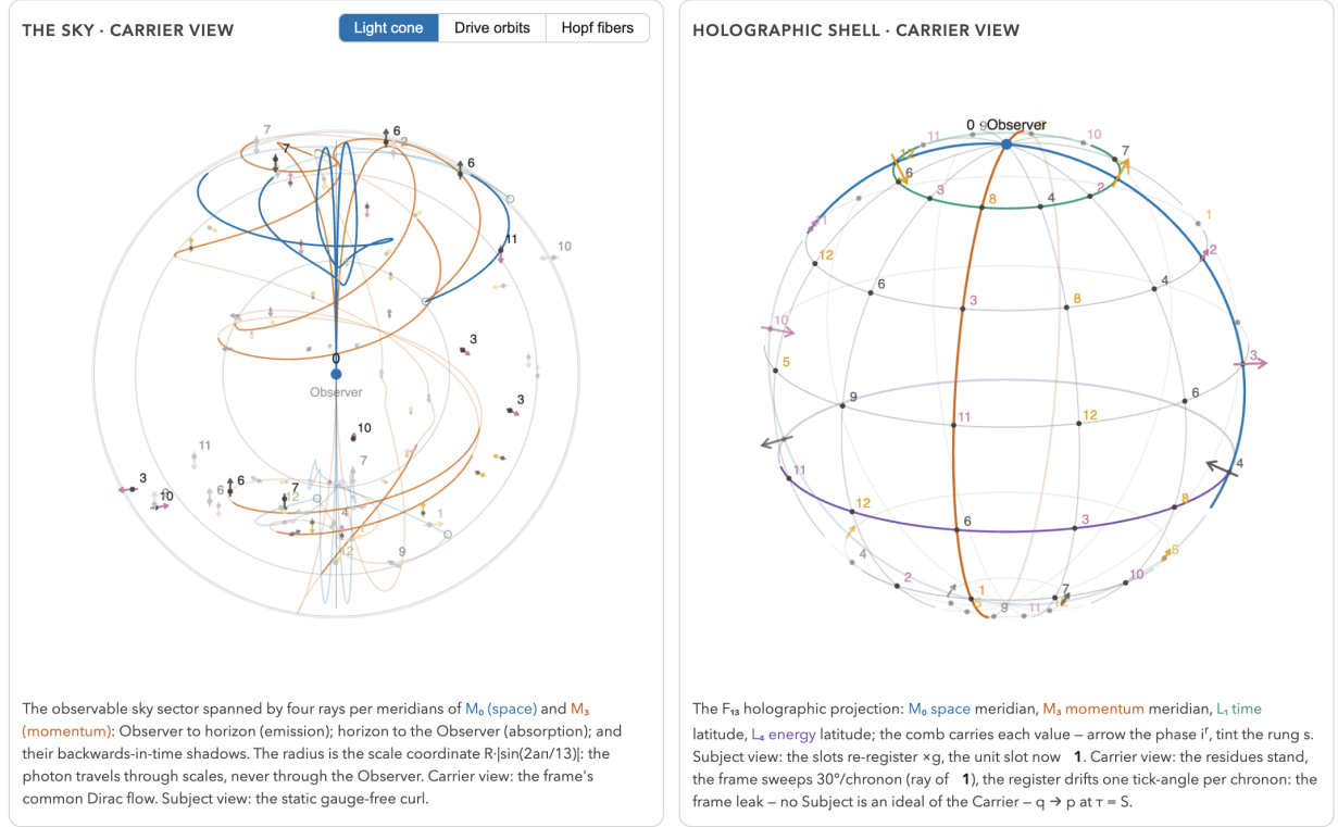
Figure 1: The laboratory (production rendering from https://frc-lab.gamma.earth/1-phase/ ): the sky (left) and the holographic encoding shell (right), one state under the Subject/Carrier toggle; the sky's representation toggle (light cone / drive orbits / Hopf fibers) visible in the panel header. Every drawn law of §6–§8 is on this page; the rendering itself is verified by verify-render (20 checks).
