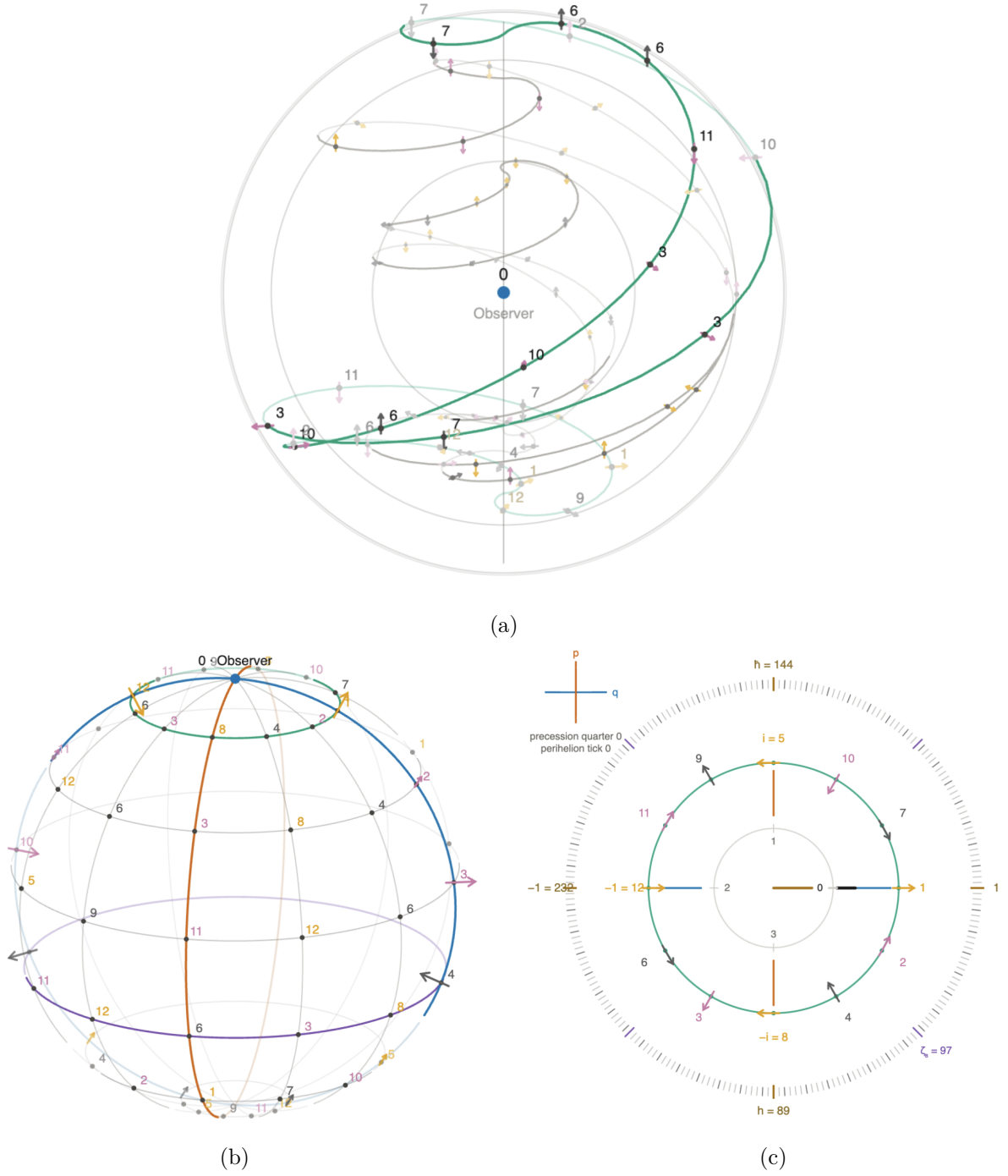
Figure 5: The three panels, one state, Subject view. (a) The sky: \kappa = 3 nested shells on the radial ladder, the Observer central, the 72-node field with each cell's phase arrow and rung tint (drive-orbit representation). (b) The holographic shell: the \mathbb{F}_{13} sphere with its graticule, the frame's prime (blue) and quarter (red) meridians, the L_1 time latitude (green) carrying the register comb, the L_4 energy latitude (purple), the Observer at the pole. (c) The phase chart: the Carrier ring of 232 ticks with the action poles \hbar = 144 and h = 89 ( \hbar + h = \Omega , A4) and the octant marks \zeta_8 = 97 ( \zeta_8^2 = h ); the Subject ring C_{12} with the quarter i = 5 , -i = 8 ; the fold clock r = \tau \bmod 4 ; the q/p dial with the two leak counters, the precession quarter and the perihelion tick (C7).
