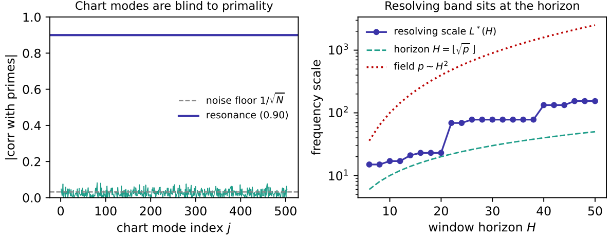
Figure 3: The equidistribution obstruction and the resolving scale. Left : the correlation of the prime indicator with each multiplicative-chart mode at p = 1009 hugs the noise floor 1/\sqrt{N} across all modes, while the units-chart resonance reaches 0.90 (Numerical Observation 6.5). Right : the resolving threshold L^*(H) tracks the horizon H = \lfloor \sqrt{p} \rfloor and lies far below the field scale p \sim H^2 , reflecting prime-power thresholds (Numerical Observation 6.3).
