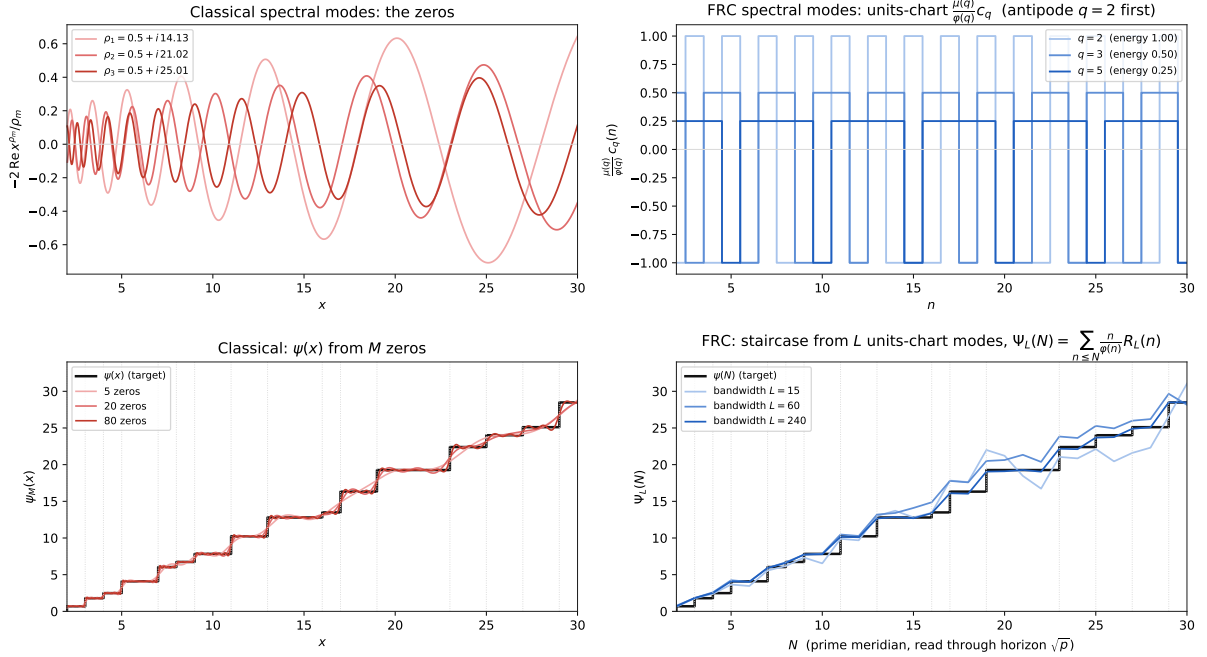
Figure 2: Prime-counting function from spectral modes: classical zeros (left) and FRC units-chart modes (right). Top : the spectral modes — the lowest zeros -2 \operatorname{Re} x^{\rho_m}/\rho_m and the units-chart modes \frac{\mu(q)}{\varphi(q)} c_q in energy order ( q = 2 , the antipode/oddness, first). Bottom : the staircase emerging — \psi_M(x) from M zeros and \Psi_L(N) = \sum_{n \leq N} \frac{\mu(n)}{\varphi(n)} R_L(n) from bandwidth L , both converging to the same \psi . The FRC wiggle at low L is the analogue of the classical Gibbs overshoot at low M and tightens monotonically with bandwidth.
