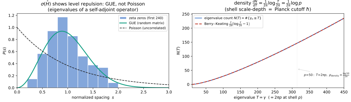
Figure 7: The zeros as eigenvalues of the scale-evolution operator \hat{H} , with \sigma(\hat{H}) = \{-i(\rho - \frac{1}{2})\} . Left: the unfolded spacings show GUE level repulsion, not Poisson — the spectrum of a self-adjoint operator with chaotic dynamics. Right: the eigenvalue count N(T) lies on the Berry–Keating semiclassical \frac{T}{2\pi}(\log \frac{T}{2\pi} - 1) , i.e. density \frac{1}{2\pi} \log p , the shell scale-depth with cutoff 1\tau .
