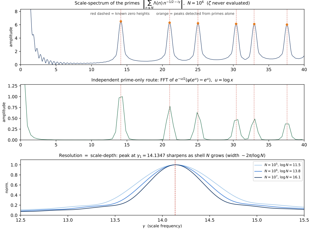
Figure 5: The spectrum of \hat{H} read from the prime side, with \zeta never evaluated. Top: the scale-spectrum of the von Mangoldt comb \left| \sum_{n \leq N} \Lambda(n) n^{-1/2 - i\gamma} \right| at N = 10^6 ; the peaks (orange) fall on the zero heights (red dashed). Middle: the independent estimator, the Fourier transform of the prime-counting fluctuation e^{-u/2}(\psi(e^u) - e^u) in the scale coordinate u = \log x , with the same peaks. Bottom: the resolving power is the scale-depth — the peak at \gamma_1 = 14.1347 sharpens as the shell N grows, width \sim 2\pi/\log N .
