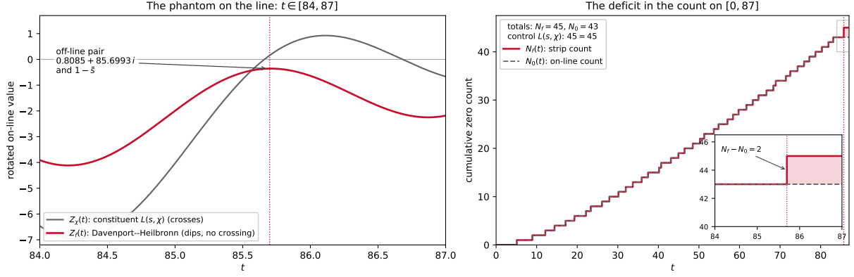
Figure 8: The Euler-product discriminator demonstrated (Numerical Observation 10.1). Left: rotated on-line values on [84, 87] : the constituent L(s, \chi) crosses zero twice (two on-line zeros), while the Davenport–Heilbronn f dips at the off-line height 85.70 without crossing — two strip zeros invisible to the line. Right: the cumulative strip count N_f(t) against the on-line count N_0(t) for f on [0, 87] : the staircases coincide until the off-line pair at t = 85.70 , where the phantom deficit N_f - N_0 = 2 opens (inset: the gap; totals 45 against 43); the identical pipeline on the constituent L(s, \chi) closes with 45 = 45 , deficit zero in every band.
