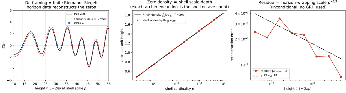
Figure 4: The de-framing function as finite Riemann–Siegel reconstruction. Left : the horizon-length sum (length \sqrt{T/2\pi} = \sqrt{p} , weight n^{-1/2} = \text{half-turn} ) tracks Z(T) through the zeros. Center : the smooth zero density equals the shell scale-depth \frac{1}{2\pi} \log p . Right : the reconstruction error follows p^{-1/4} , the horizon scale, with no hypothesis used.
