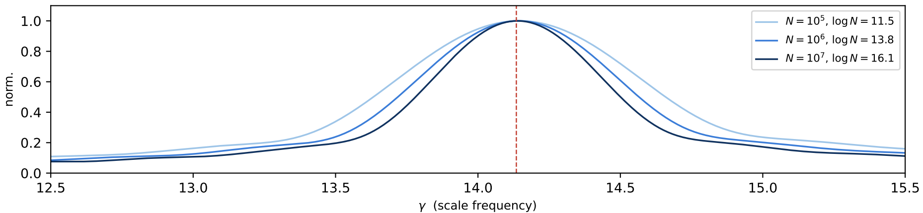
Resolution = scale-depth: peak at \gamma_1 = 14.1347 sharpens as shell N grows (width \sim 2\pi/\log N )
