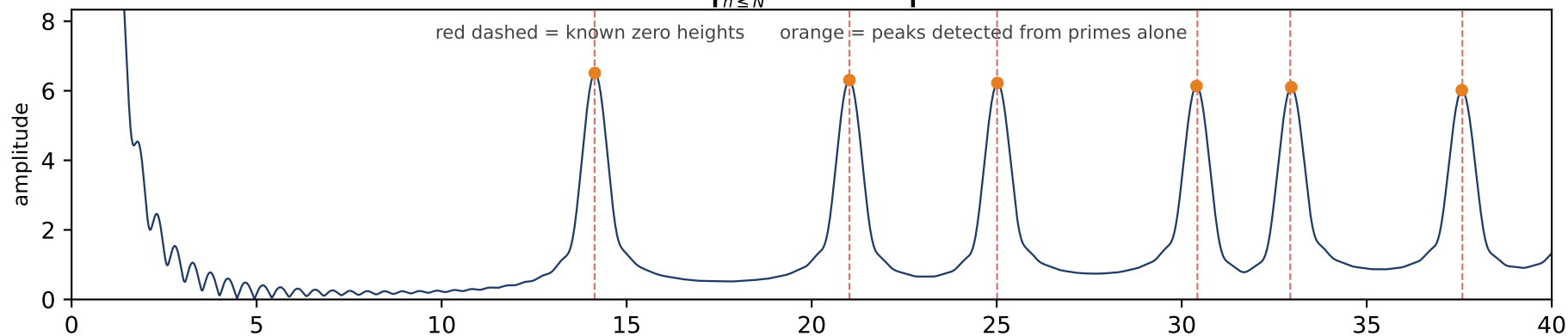
Independent prime-only route: FFT of e^{-u/2}(\psi(e^u) - e^u) , u = \log x
