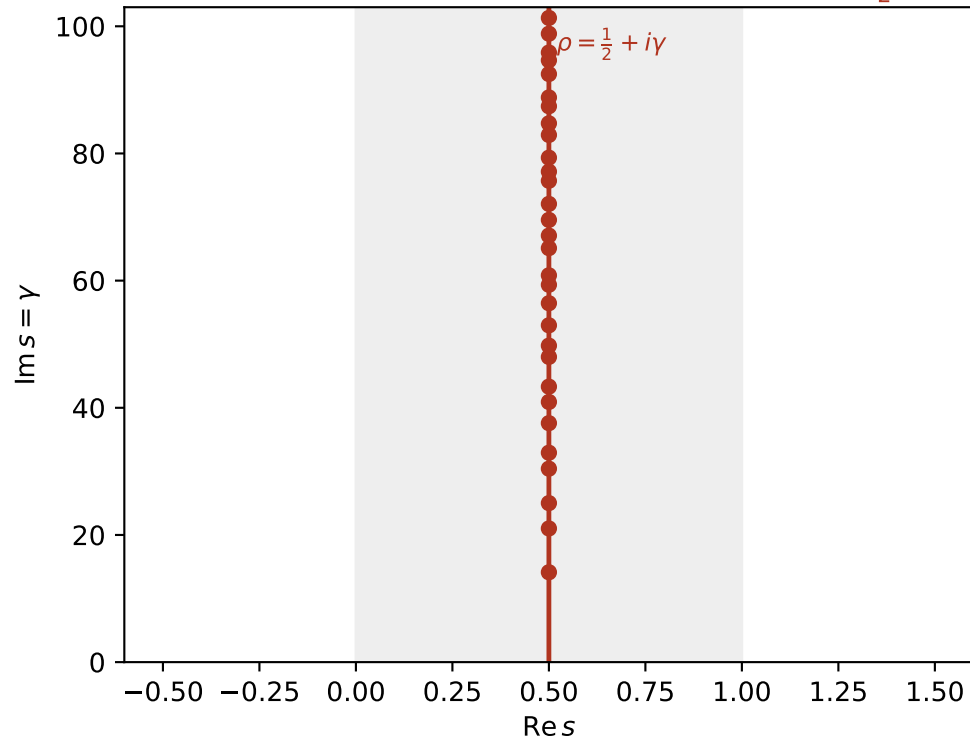
Continuum: the zero spectrum reconstructs the primes
