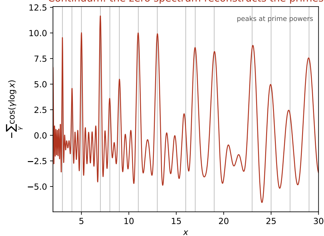
Continuum: the zero spectrum reconstructs the primes
