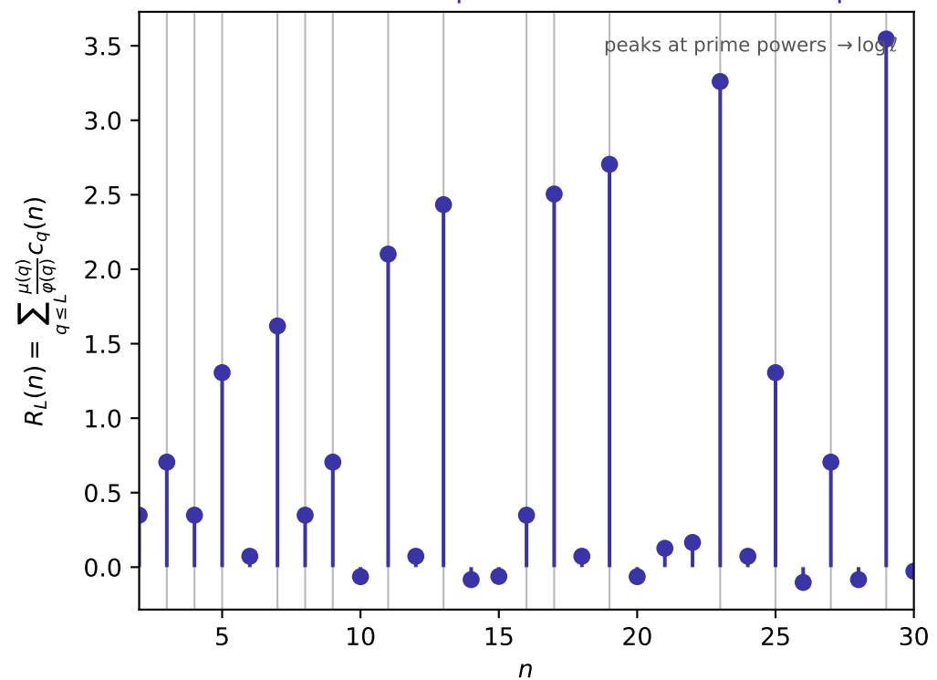
Finite: the units-chart spectrum reconstructs the primes
