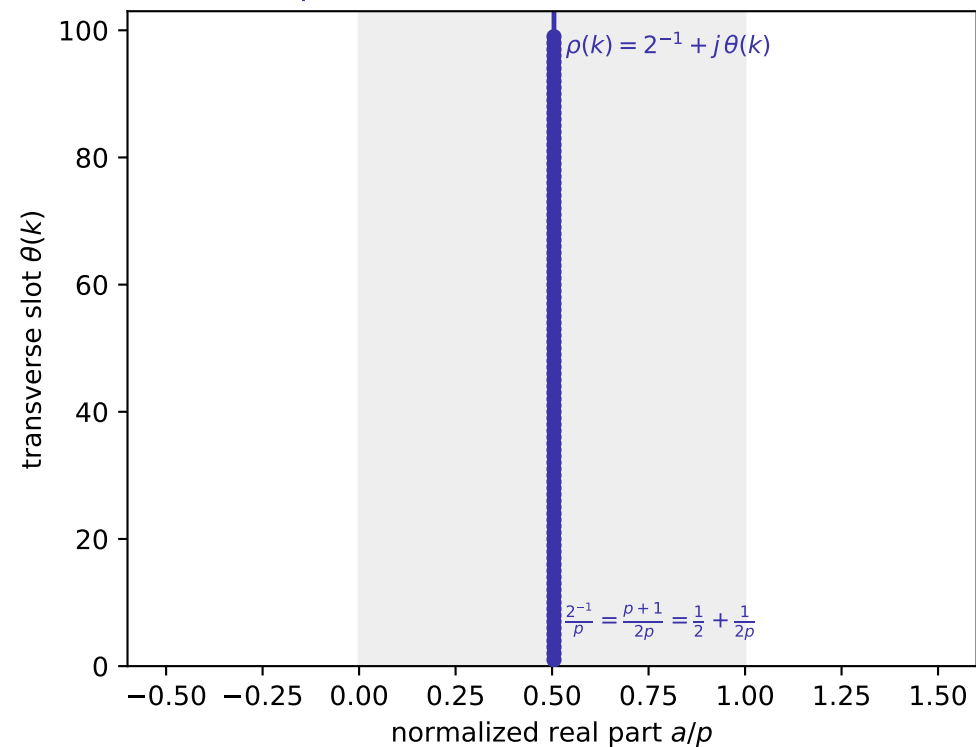
Finite: the units-chart spectrum reconstructs the primes
