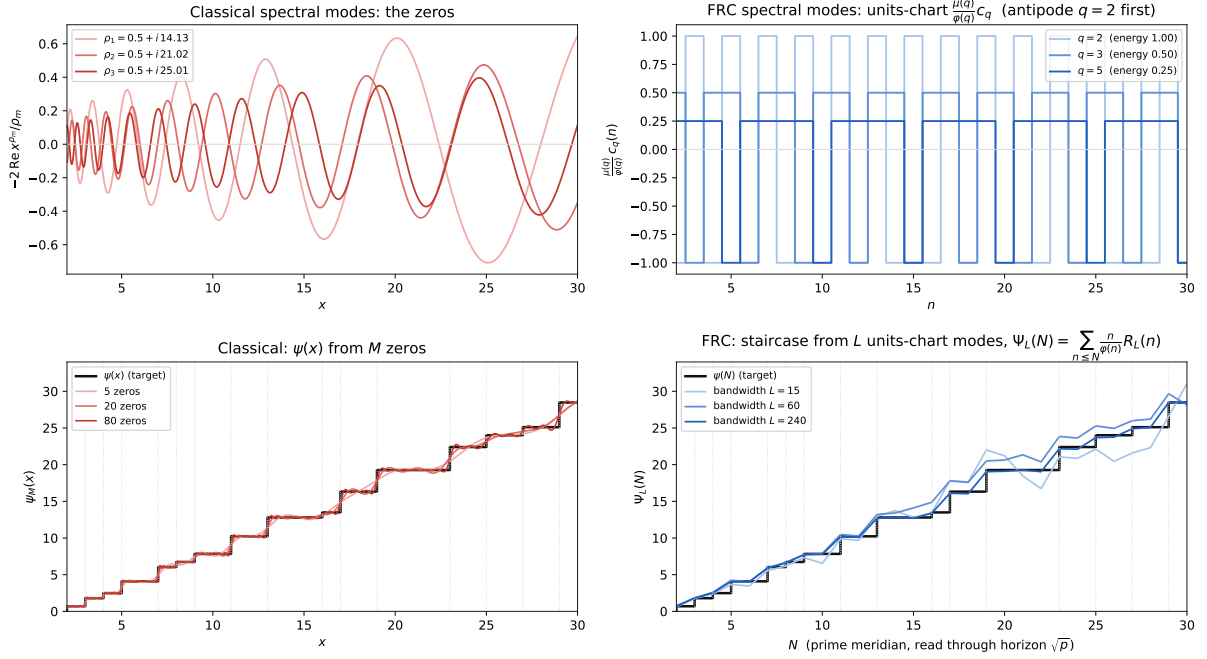
Figure 2: Prime-counting function from spectral modes: classical zeros (left) and FRC units-chart modes (right). Top : the spectral modes — the lowest zeros -2 \operatorname{Re} x^{\rho_m} / \rho_m and the units-chart modes \frac{\mu(q)}{\varphi(q)} c_q in energy order ( q = 2 , the antipode/oddness, first). Bottom : the staircase emerging — \psi_M(x) from M zeros and \Psi_L(N) = \sum_{n \leq N} \frac{n}{\varphi(n)} R_L(n) from bandwidth L , both converging to the same \psi . The FRC wiggle at low L is the analogue of the classical Gibbs overshoot at low M and tightens monotonically with bandwidth.
