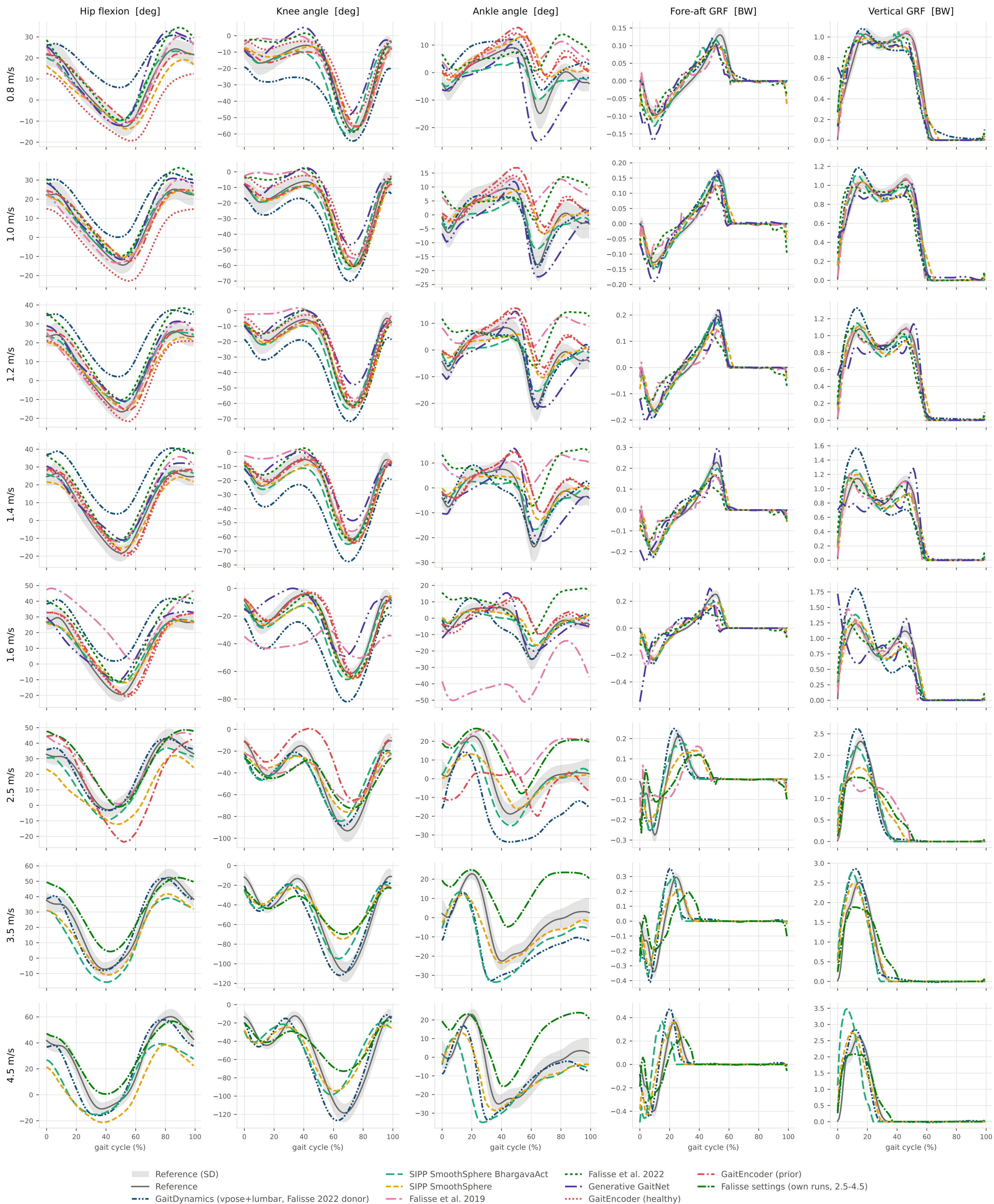
Speed sweep: generative and predictive gait models vs the experimental reference
