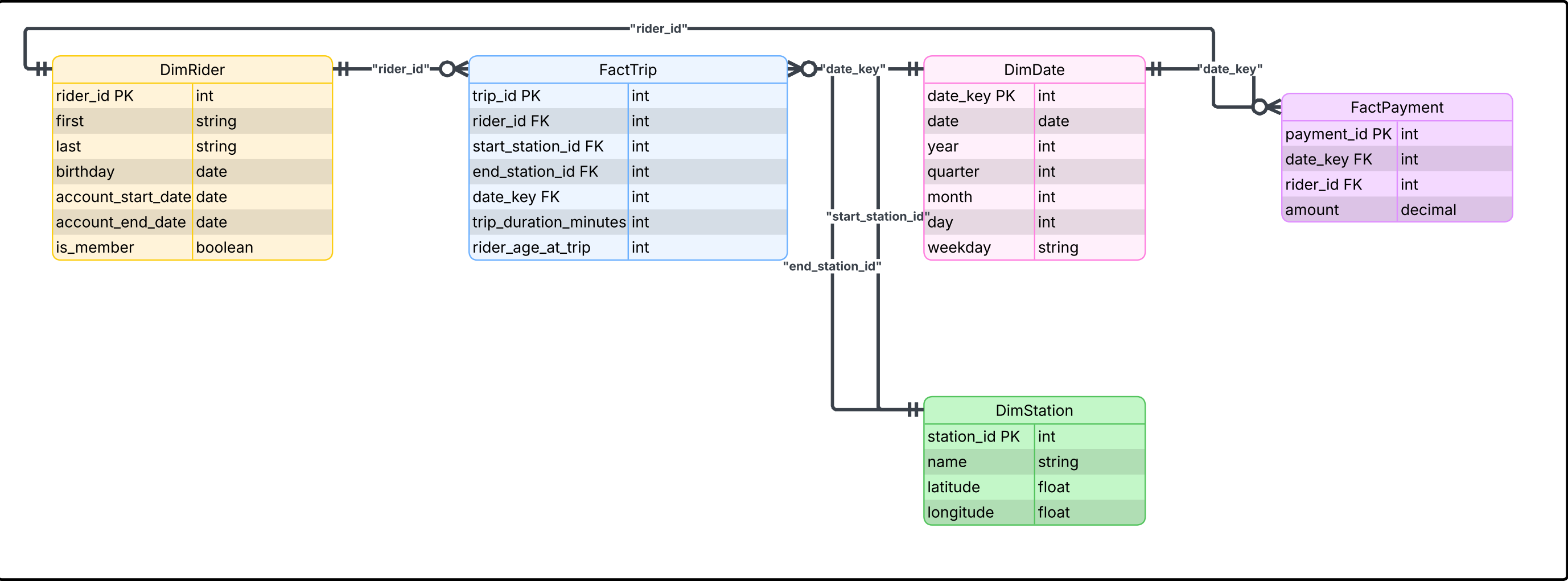
Rider Trip and Payment Star Schema
