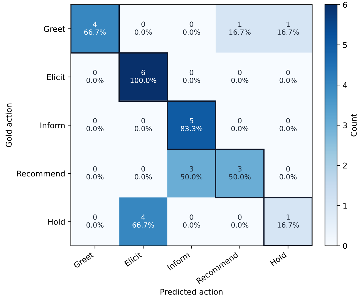
PIWM Confusion Matrix on Target-Test (n=30)
