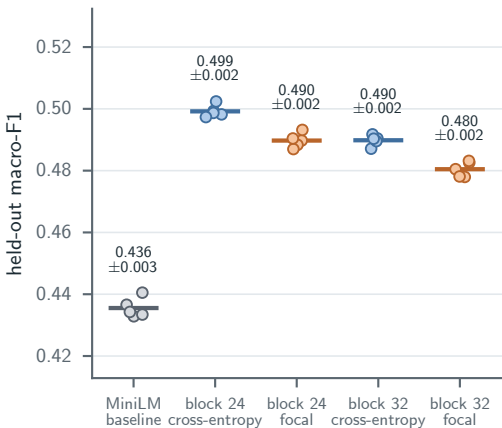
(a) Sentence classifier, 5 seeds each
