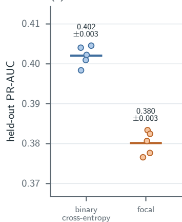
(c) Staleness PR-AUC
