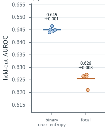
(b) Staleness AUROC
