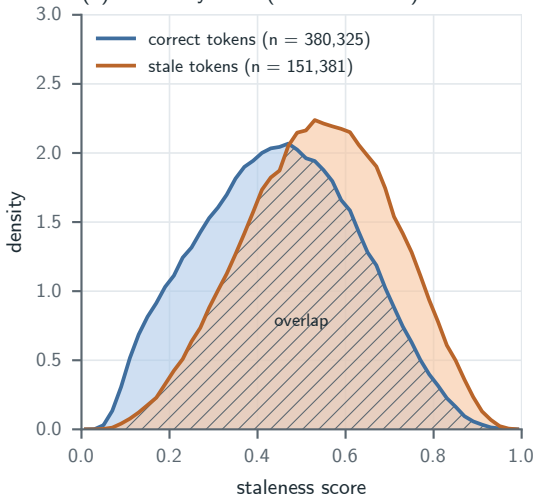
(a) Scores by label (AUROC 0.645)
