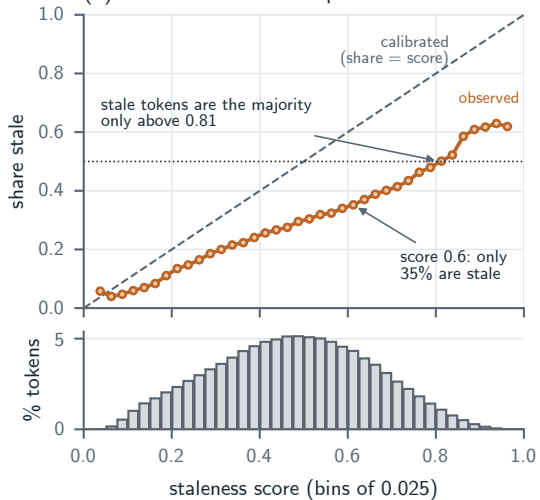
(b) Share of stale tokens per score bin
