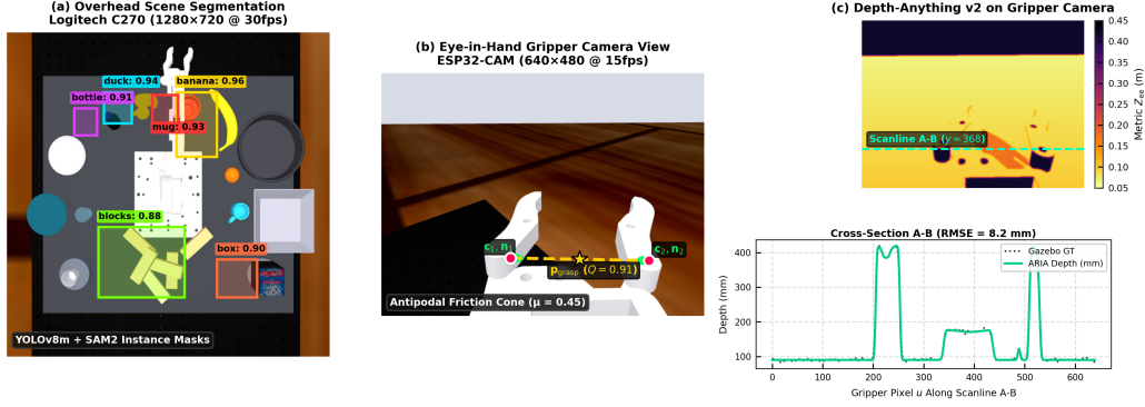
Fig. 3. Self-grounded monocular perception pipeline: (a) Dual-camera topology comprising overhead eye-to-hand Logitech C270 ( 1280 \times 720 ) and wrist-mounted eye-in-hand ESP32-CAM ( 640 \times 480 ); (b) Eye-in-hand gripper camera view with contact normal and friction cone evaluation ( \mu = 0.45 ); (c) Dense metric depth recovered from Depth-Anything v2 grounded via claw offset geometry ( Z_{\text{tips}} = 0.065 m) compared against Gazebo simulation ground truth.
