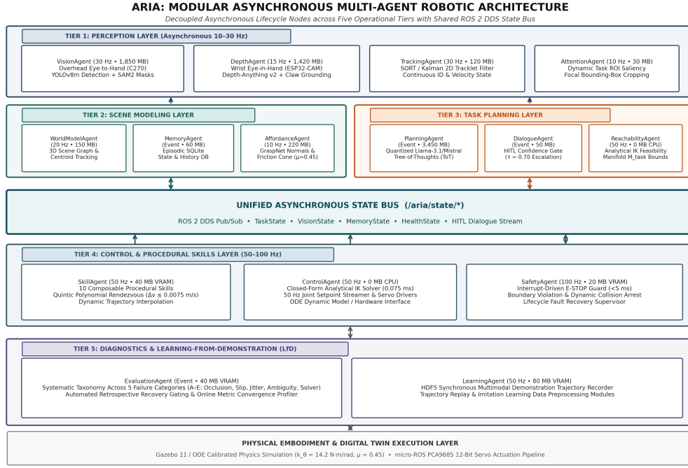
Fig. 2. Modular asynchronous multi-agent architecture of Project ARIA. The system is organized across five functional tiers matching Table IV: (1) Perception (VisionAgent, DepthAgent, TrackingAgent, AttentionAgent); (2) Scene Modeling (WorldModelAgent, MemoryAgent, AffordanceAgent); (3) Task Planning (PlanningAgent, DialogueAgent, ReachabilityAgent); (4) Control & Skills (SkillAgent, ControlAgent, SafetyAgent); and (5) Diagnostics & LfD (EvaluationAgent, LearningAgent).
