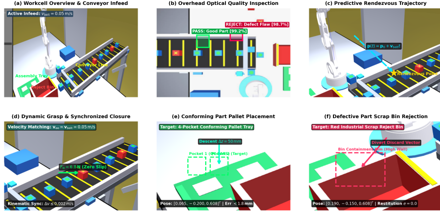
Fig. 8. Full-system simulated conveyor sorting demonstration across six sequential execution phases in the Gazebo workcell: (a) Simulated workcell overview; (b) Overhead optical defect inspection classifying conforming (PASS) vs. defective (REJECT) workpieces; (c) Predictive rendezvous trajectory generation equating arm transit time with belt displacement; (d) Dynamic grasp acquisition with feedforward velocity matching ( v_{ee} \approx v_{belt} ); (e) Conforming workpiece palletizing into 4-pocket tray ( RMSE = 1.14 mm); (f) Defective workpiece transfer and scrap bin rejection (3.8 s reject sub-motion, 14.0–36.6 s full conveyor cycle).
