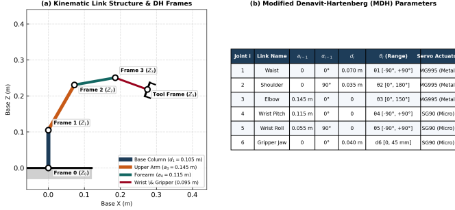
Fig. 1. Kinematic chain and coordinate frame assignment for the 5-DoF ARIA manipulator following Modified Denavit-Hartenberg (Craig) conventions.
