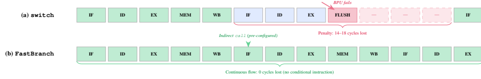
Figure 1. CPU pipeline comparison. (a) With switch : a BPU misprediction triggers a pipeline flush, wasting 14–18 cycles. (b) With FastBranch : there is no conditional instruction; the indirect branch is pre-configured, and the pipeline flows without interruption.
