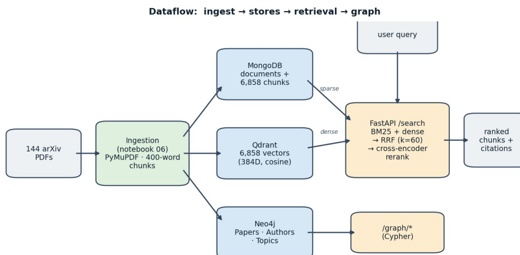
Figure 1. System dataflow: ingest → stores (MongoDB / Qdrant / Neo4j) → hybrid retrieval → graph.
