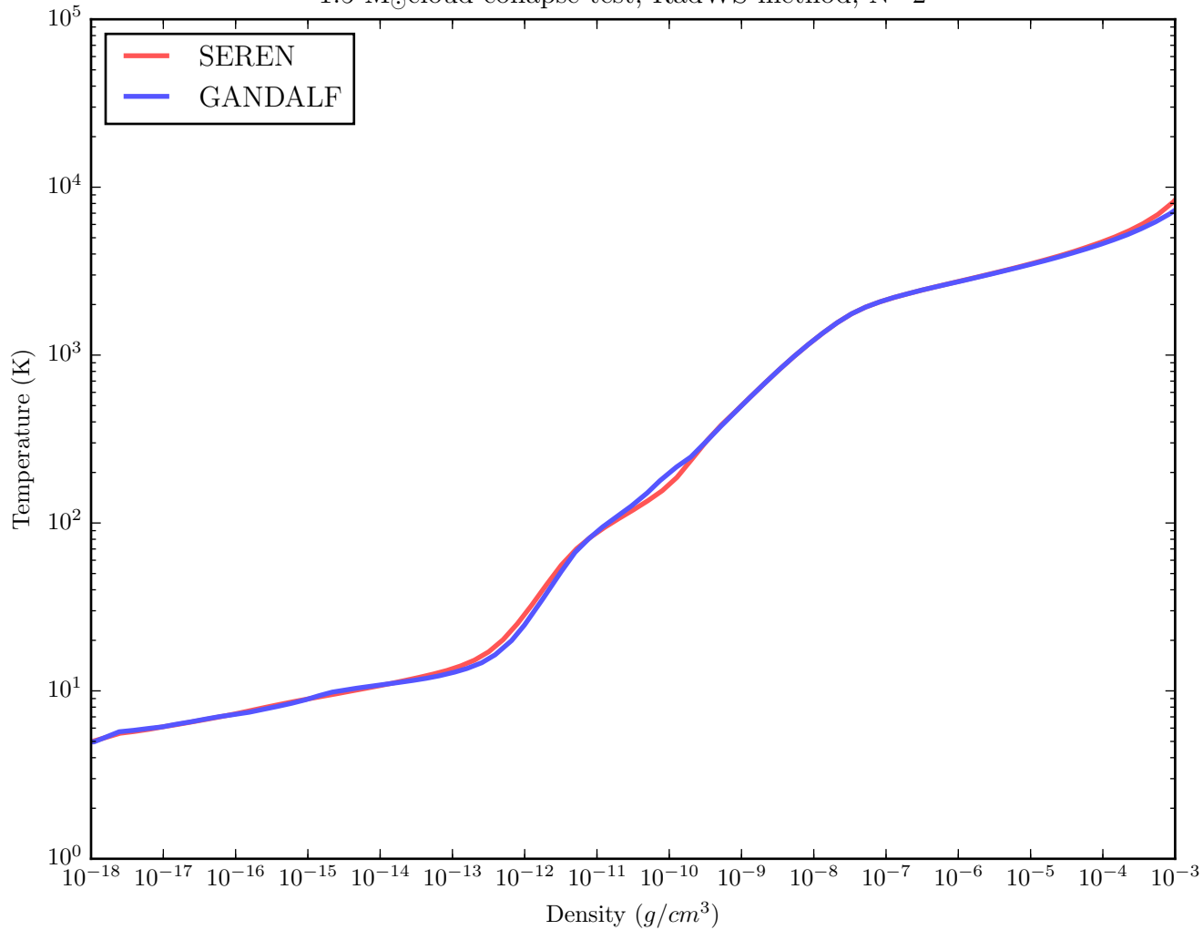
1.5 M_{\odot} cloud collapse test, RadWS method, N=2^{20}
