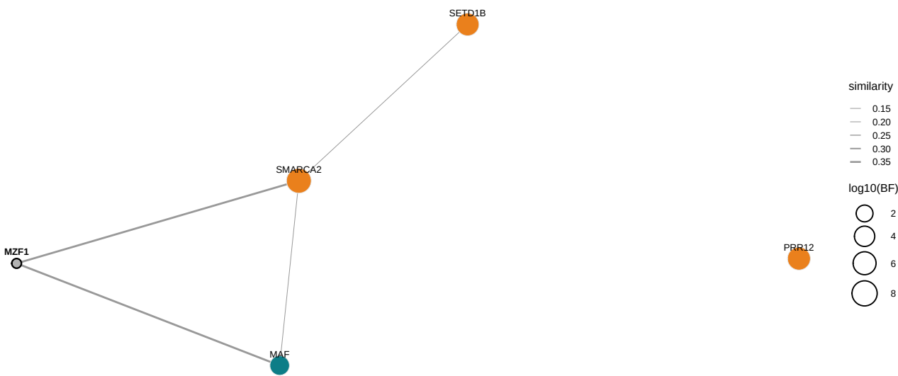
GO similarity of ASD genes (n = 4)
