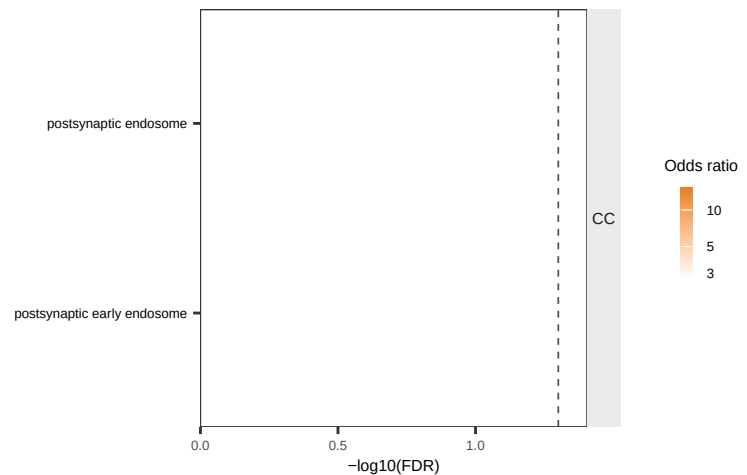
SynGO enrichment (P < 0.05)
