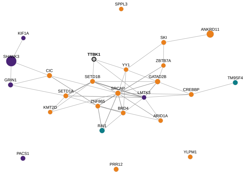
GO similarity of ASD genes (n = 27)
