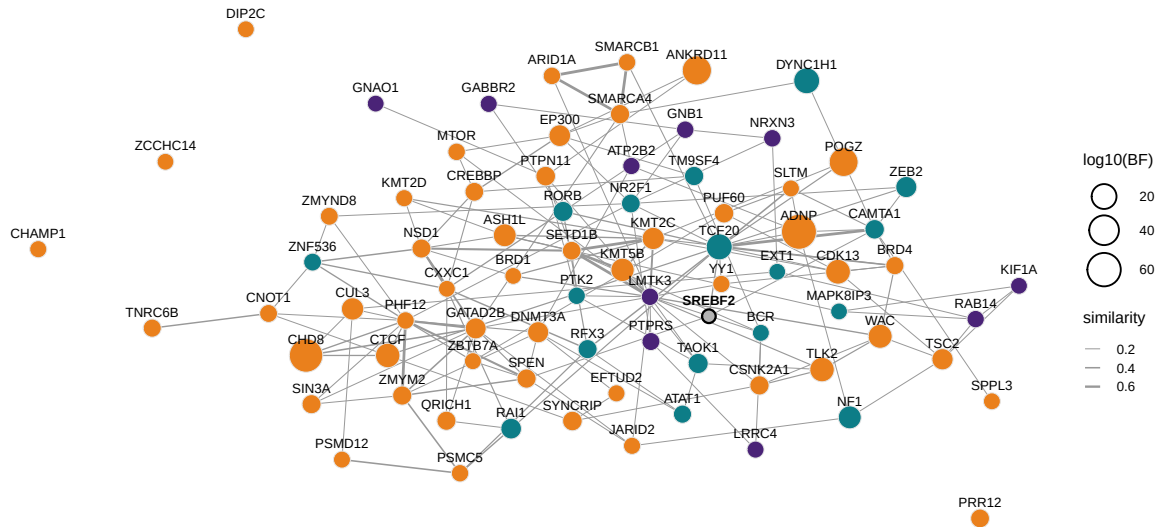
GO similarity of ASD genes (n = 78)
