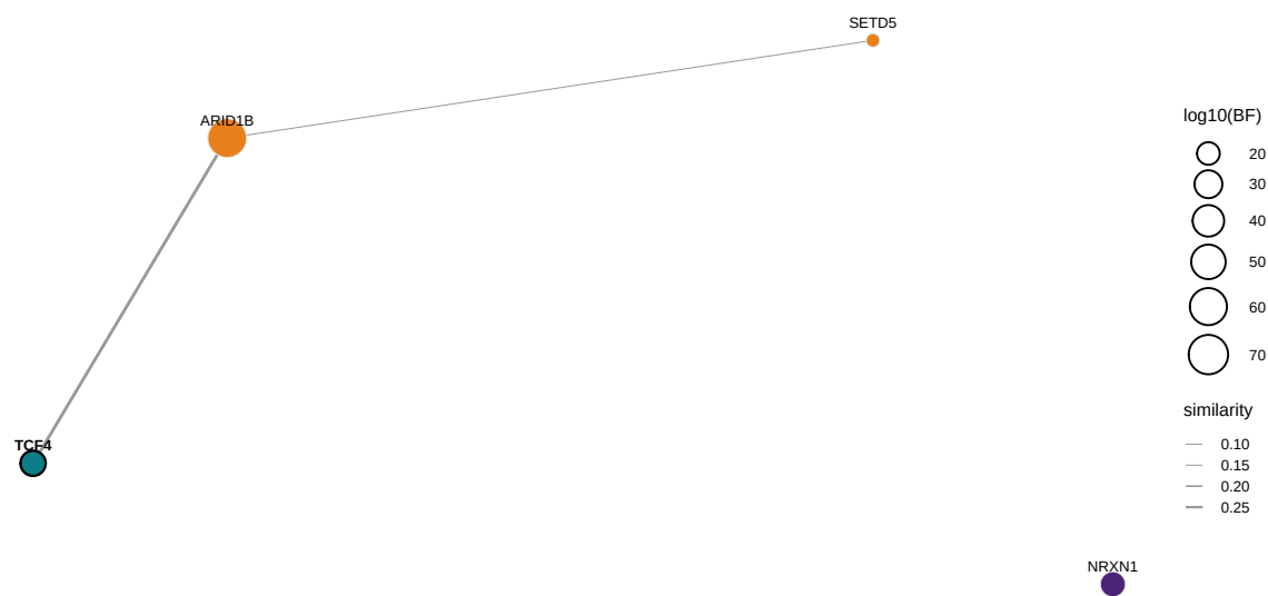
GO similarity of ASD genes (n = 4)
