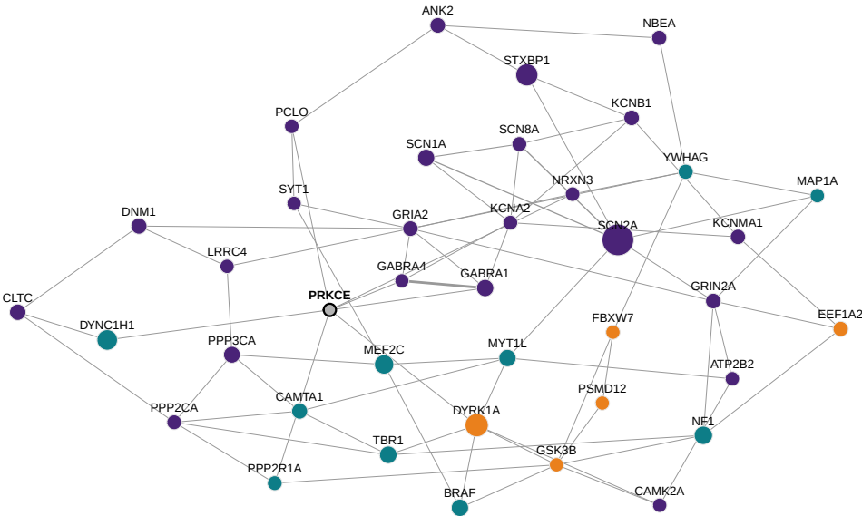
GO similarity of ASD genes (n = 38)
