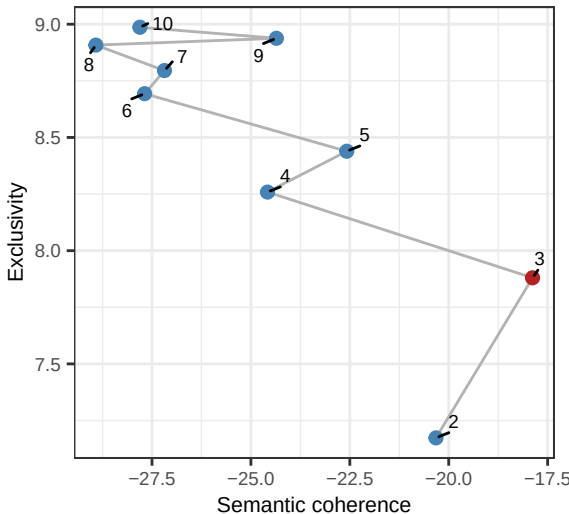
Coherence vs exclusivity tradeoff
