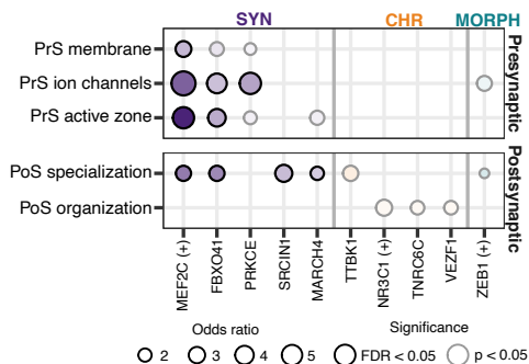
a Module enrichment for SynGO HotNets
