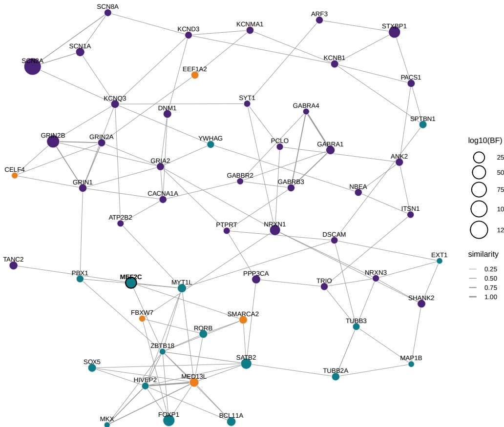
ASD Genes in MEF2C
