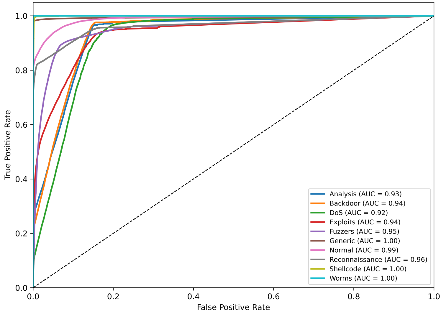
Multi-class ROC (One-vs-Rest)
