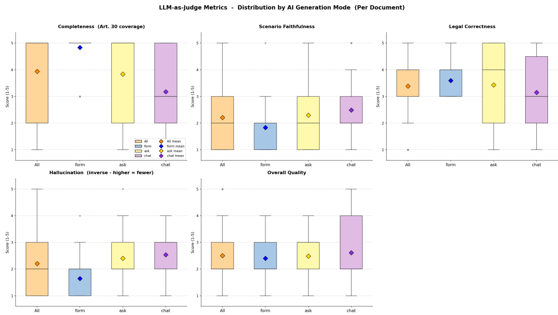
Figure 4.12: Distributions of the five LLM-as-Judge dimensions by mode (full sample n = 113 , scale 1–5).
