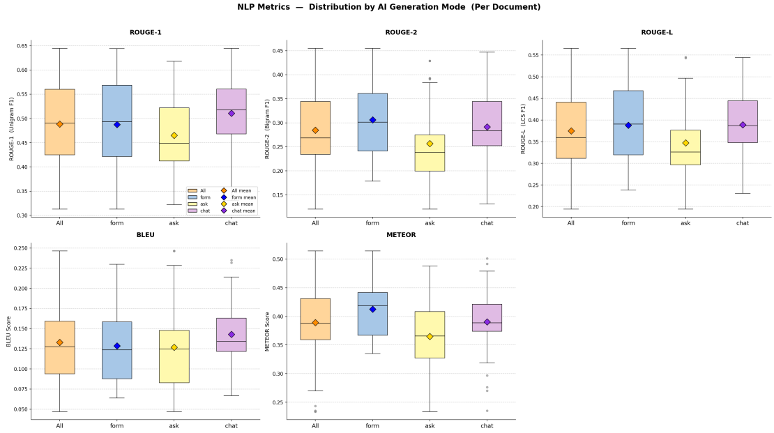
Figure 4.8: Document-level distributions of BLEU, ROUGE-1/2/L, and METEOR by mode (full sample n = 113 ). Boxes show the interquartile range; the diamond marks the mean.
