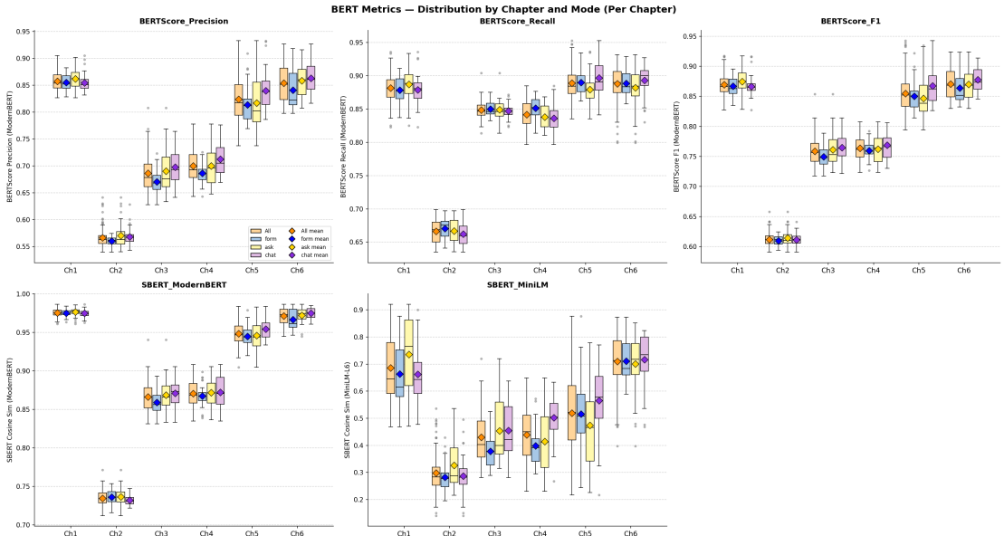
Figure 4.11: Chapter-level distributions of BERTScore Precision / Recall / F1 and SBERT cosine similarity (ModernBERT) by mode (full sample n = 113 ).
