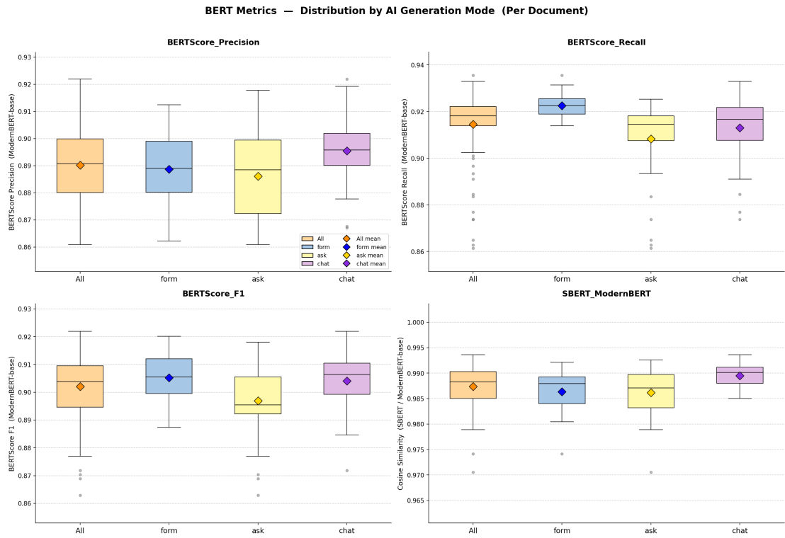
Figure 4.9: Document-level distributions of BERTScore Precision / Recall / F1 and SBERT cosine similarity (ModernBERT) by mode (full sample n = 113 ).
