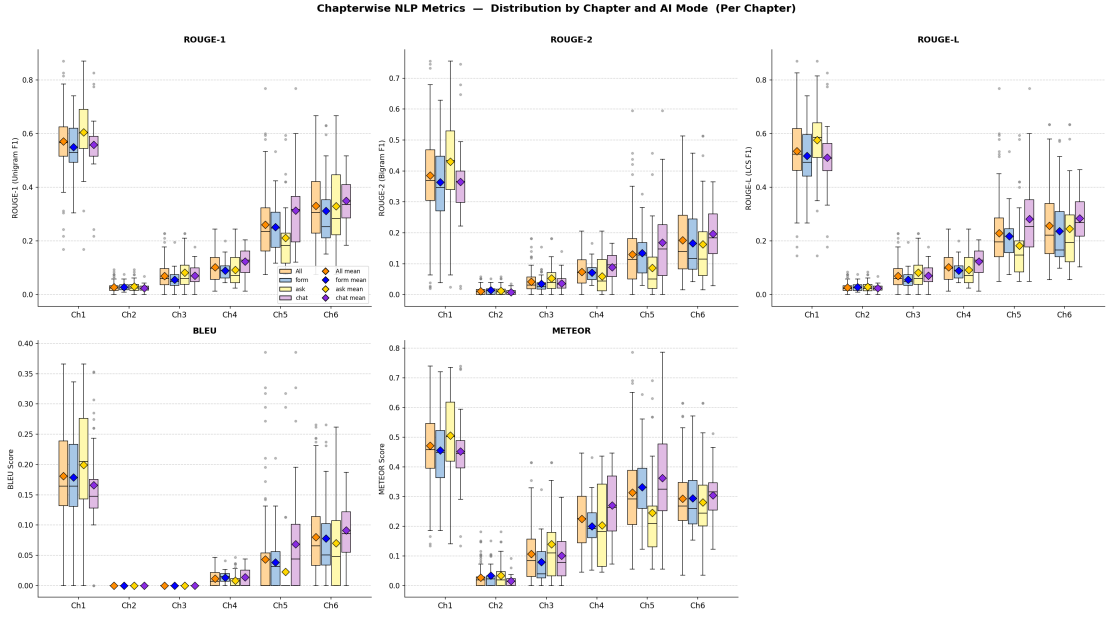
Figure 4.10: Chapter-level distributions of BLEU, ROUGE-1/2/L, and METEOR by mode (full sample n = 113 ).
