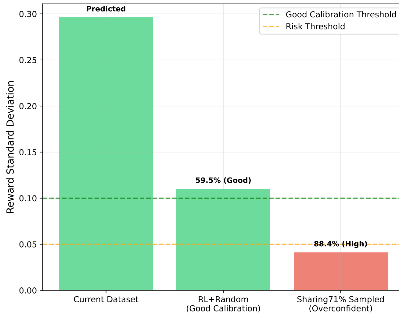
Confidence Calibration Prediction Matrix
