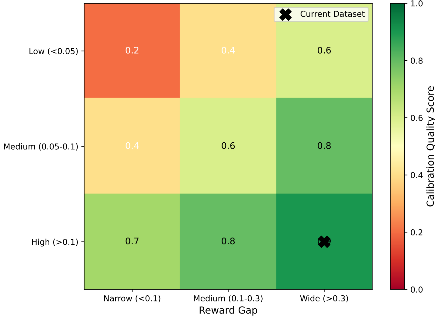
Confidence Calibration Prediction Matrix
