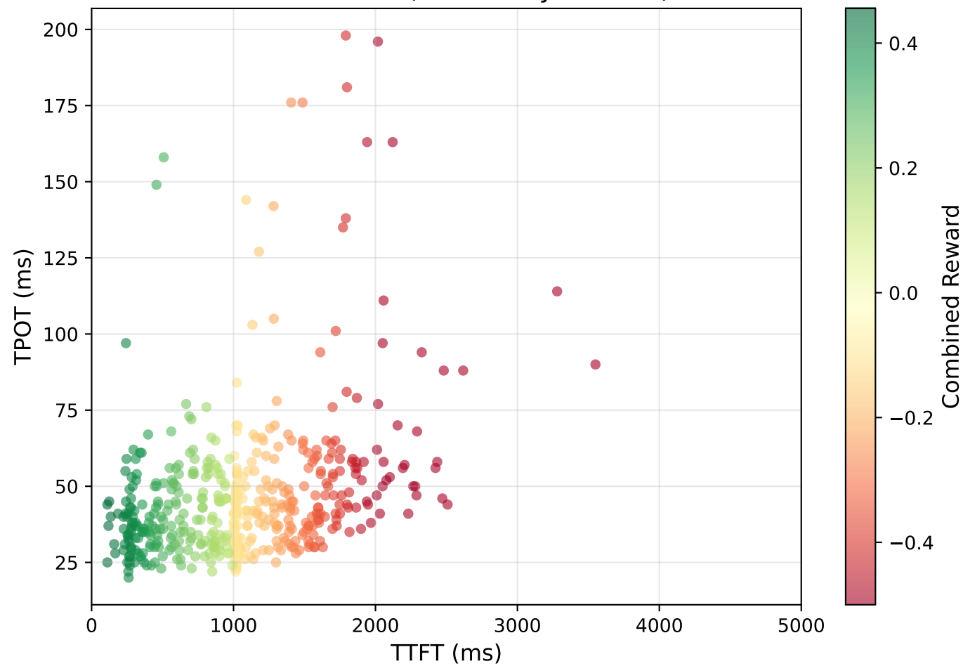
TTFT vs TPOT (colored by Reward)
