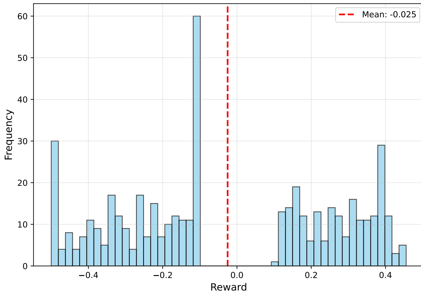
Overall Reward Distribution
