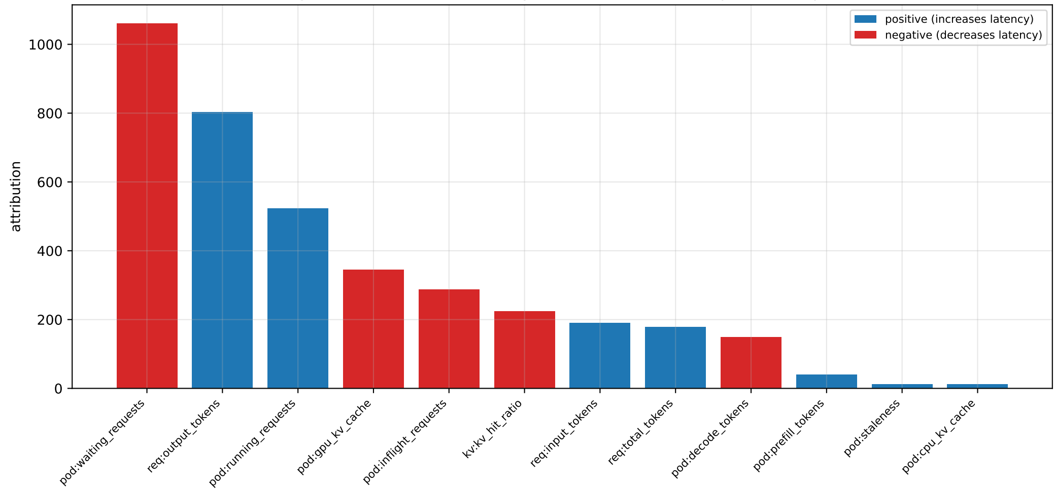
Integrated Gradients for Latency Prediction (combined: pod, kv, request)
