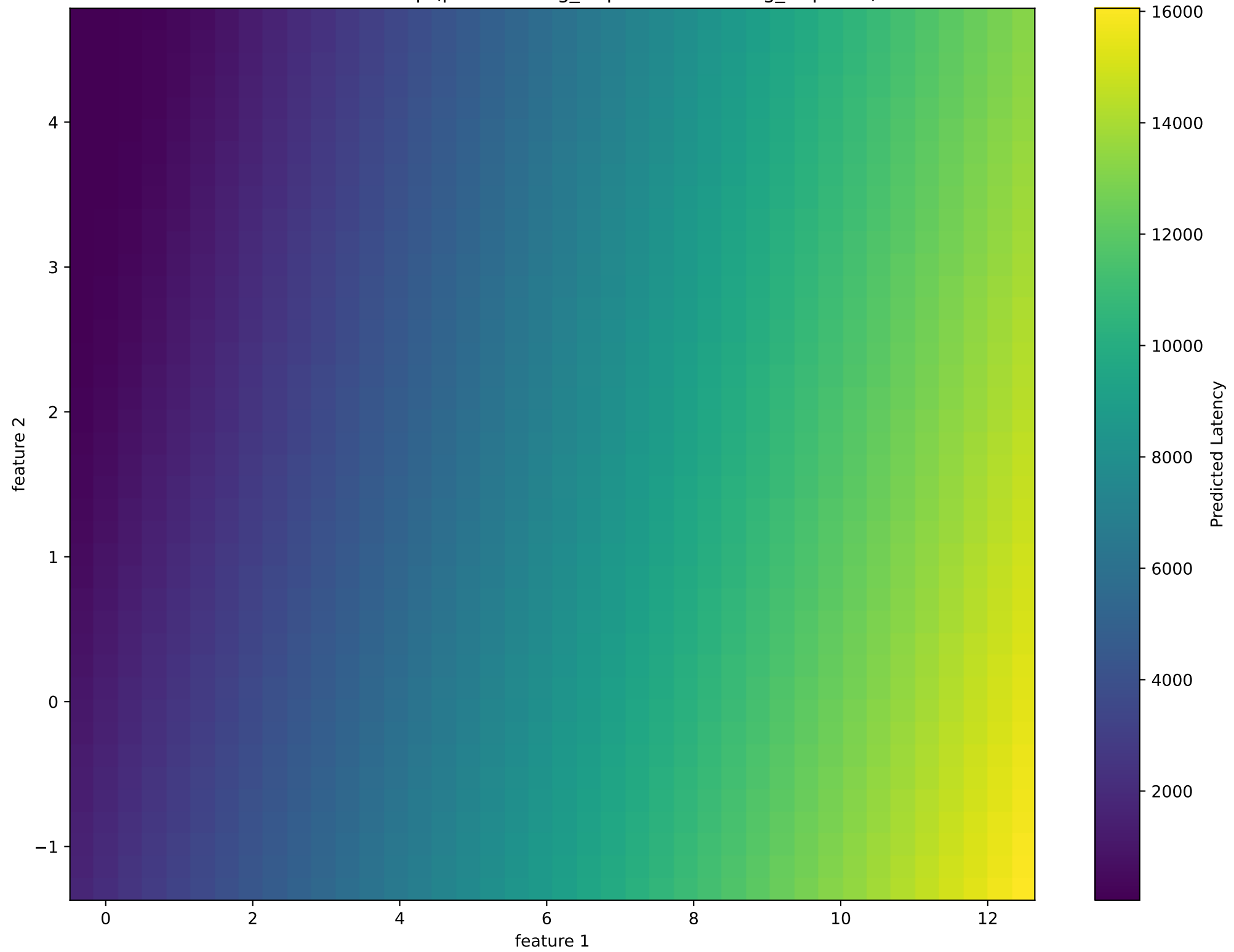
Interaction heatmap (pod0 waiting_requests vs running_requests)
