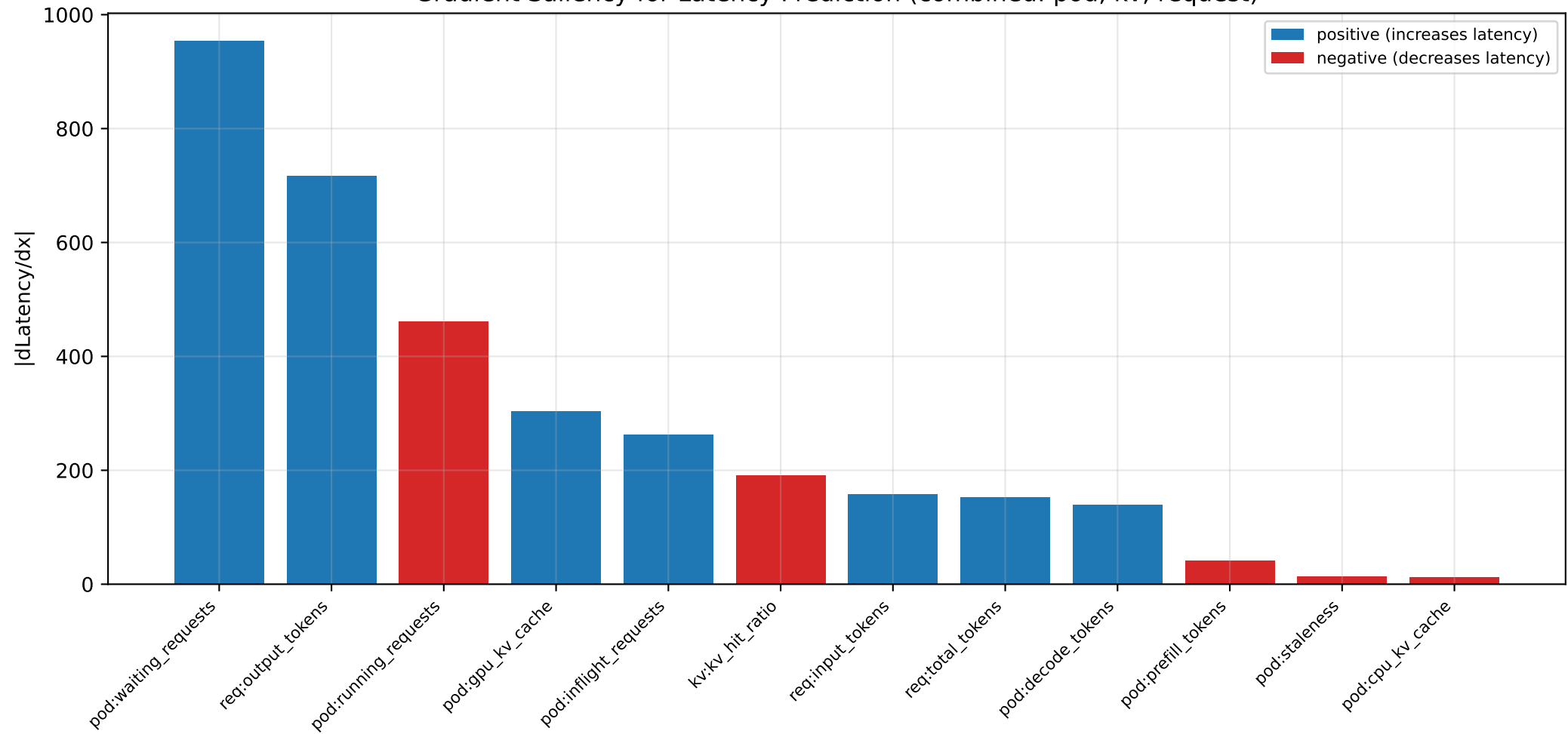
Gradient Saliency for Latency Prediction (combined: pod, kv, request)
